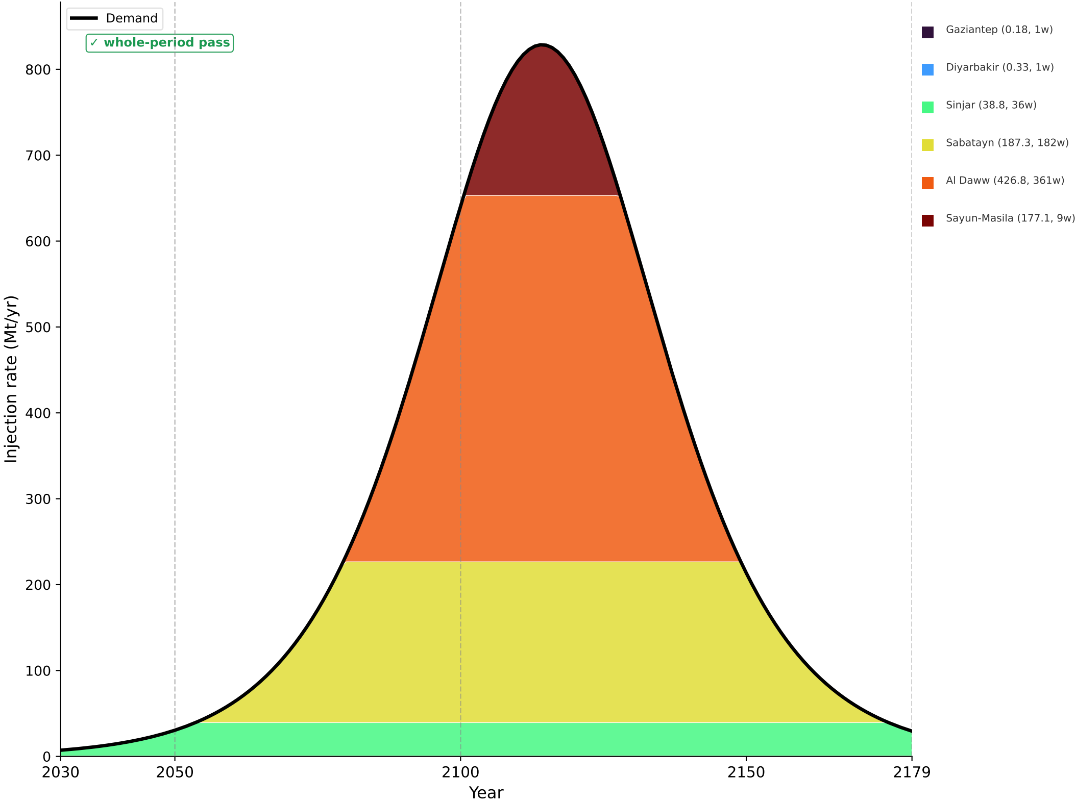
Logistic
