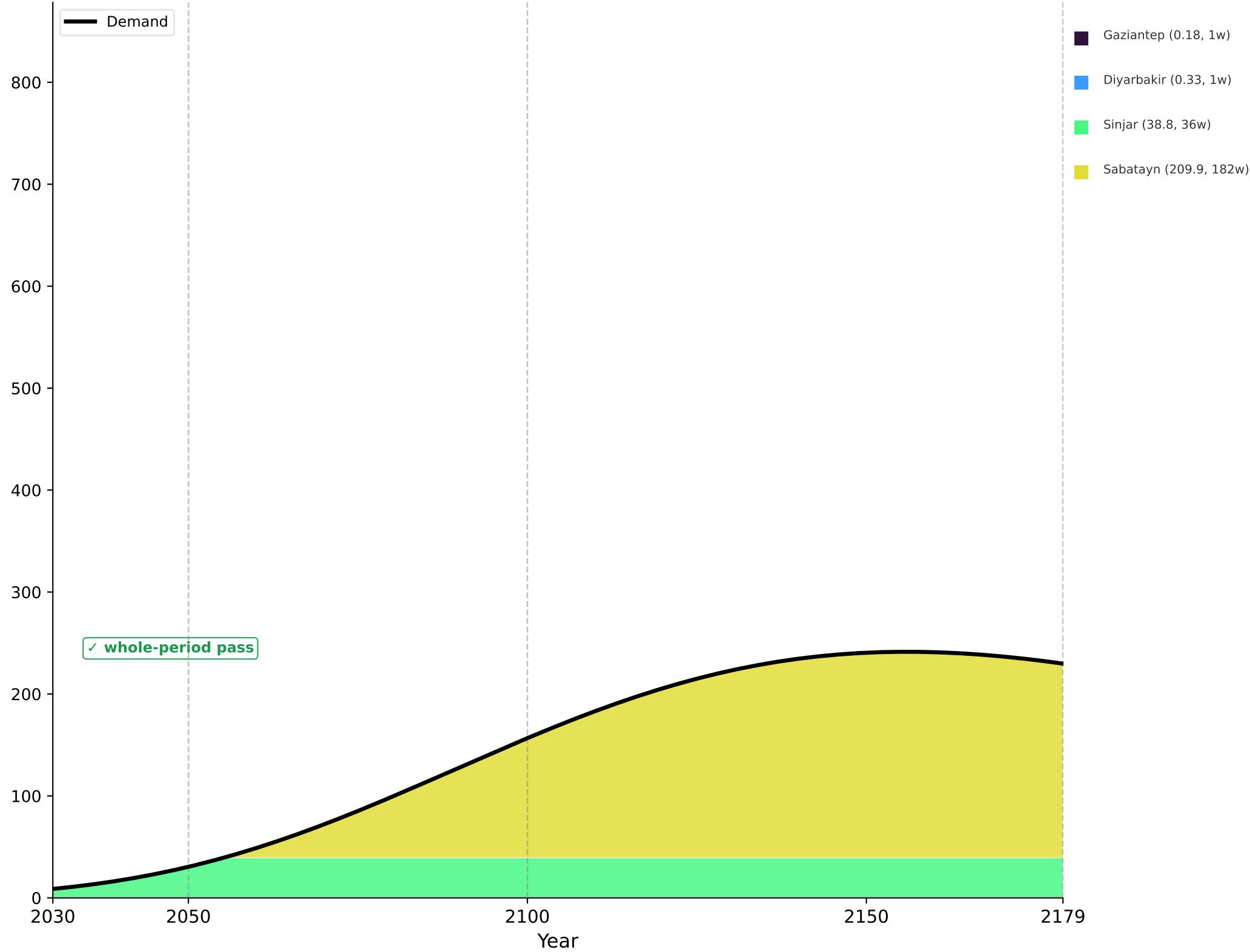
Gompertz
