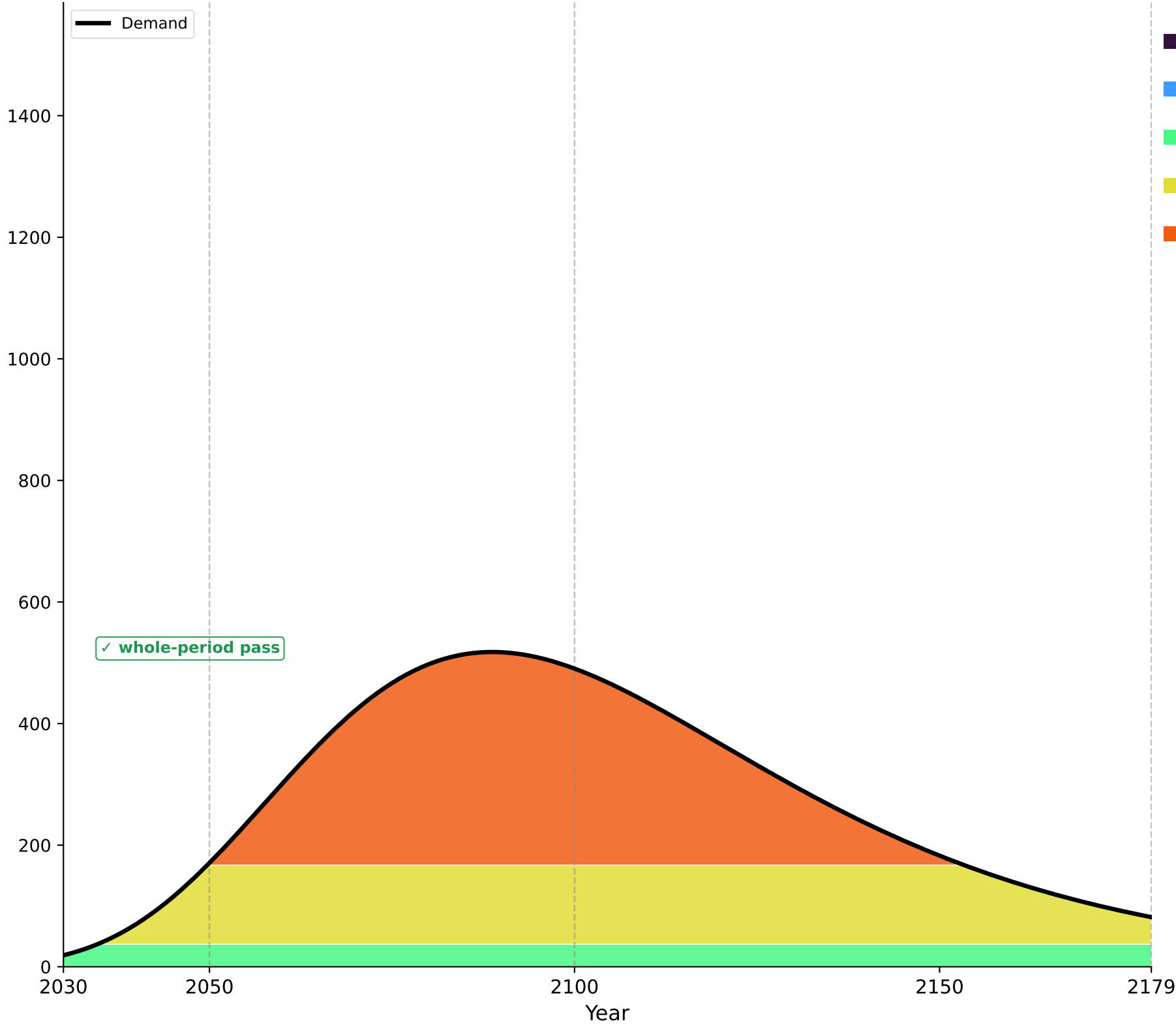
Gompertz
