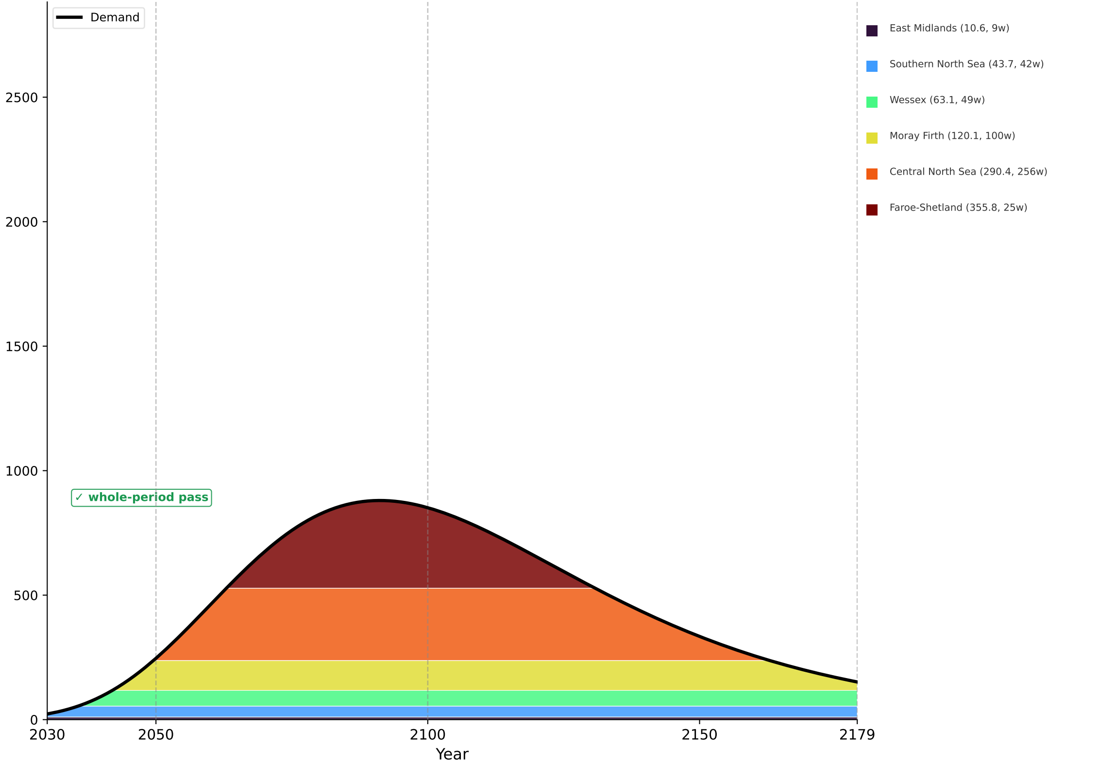
Gompertz
