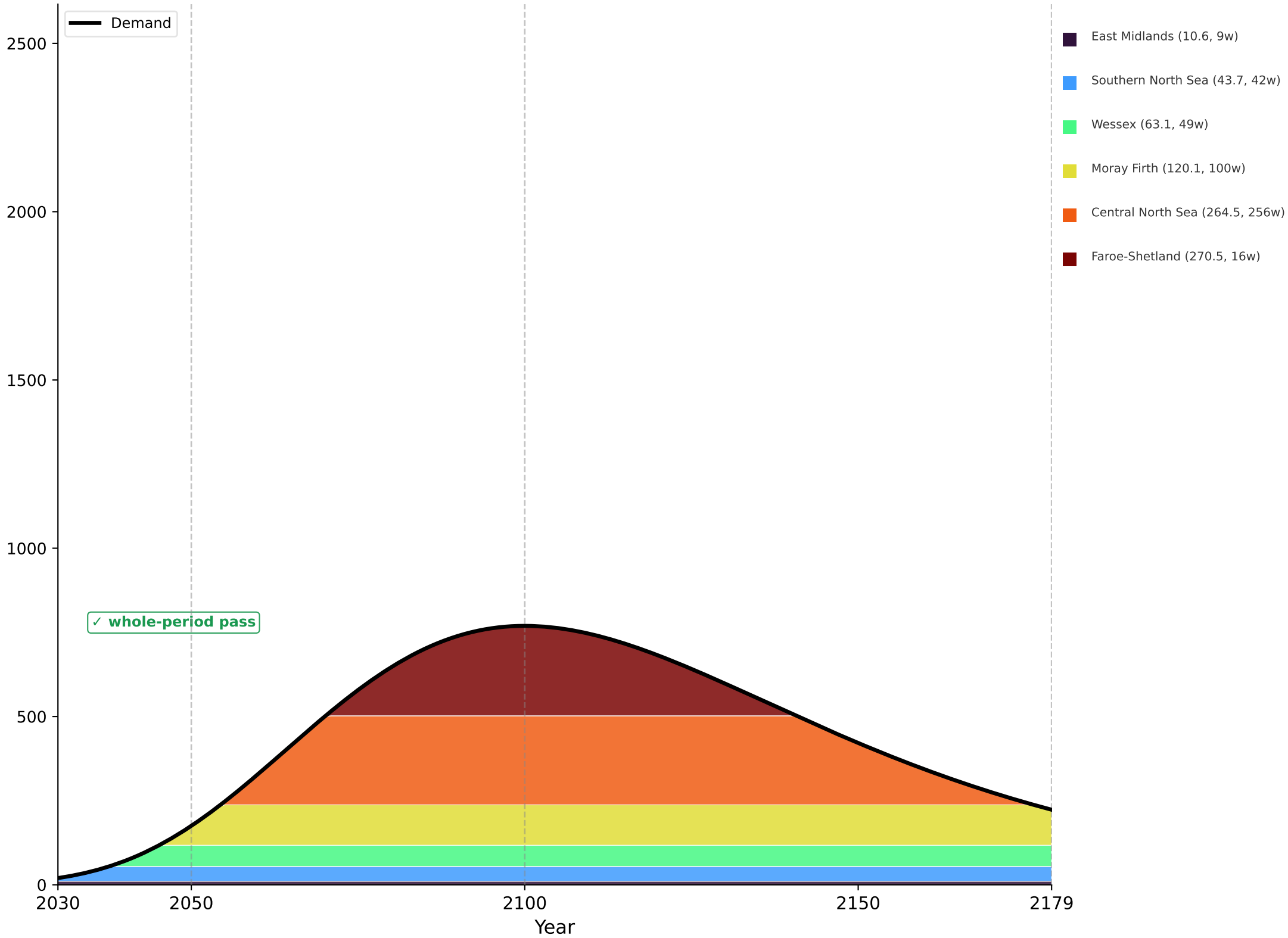
Gompertz
