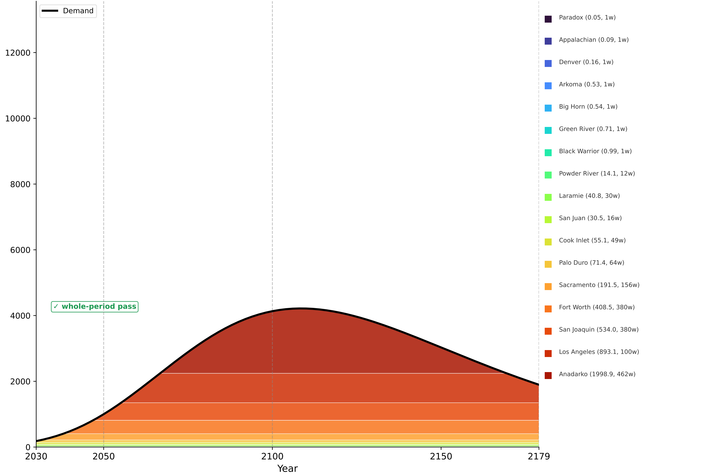
Gompertz
