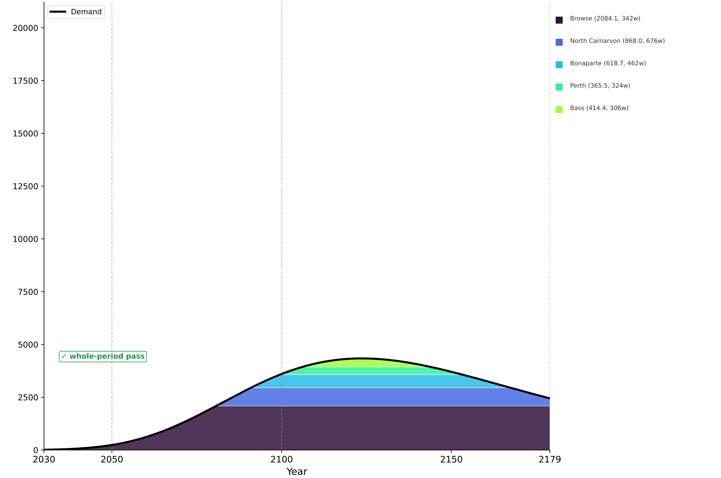
Gompertz
