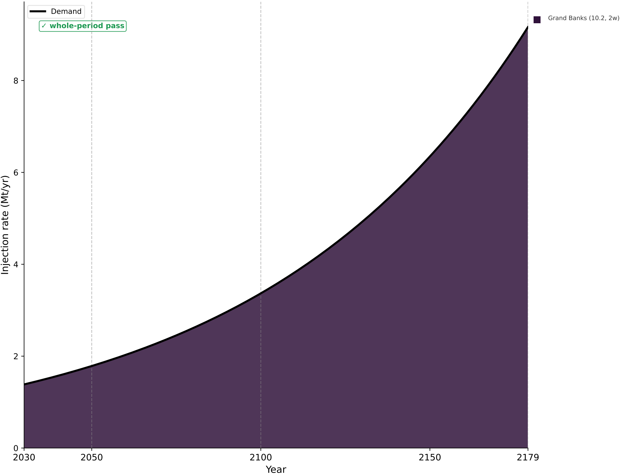
Logistic
