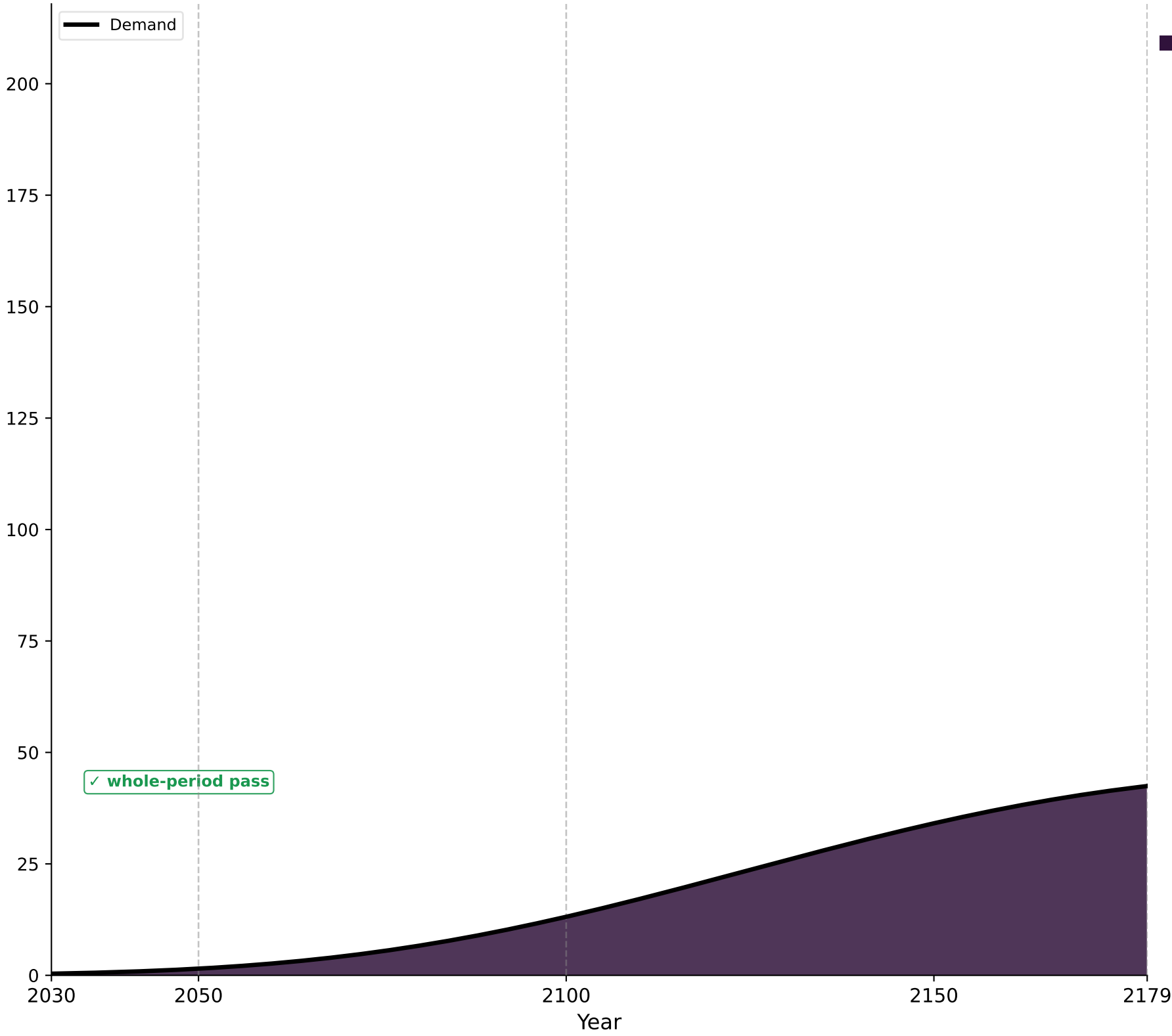
Gompertz
