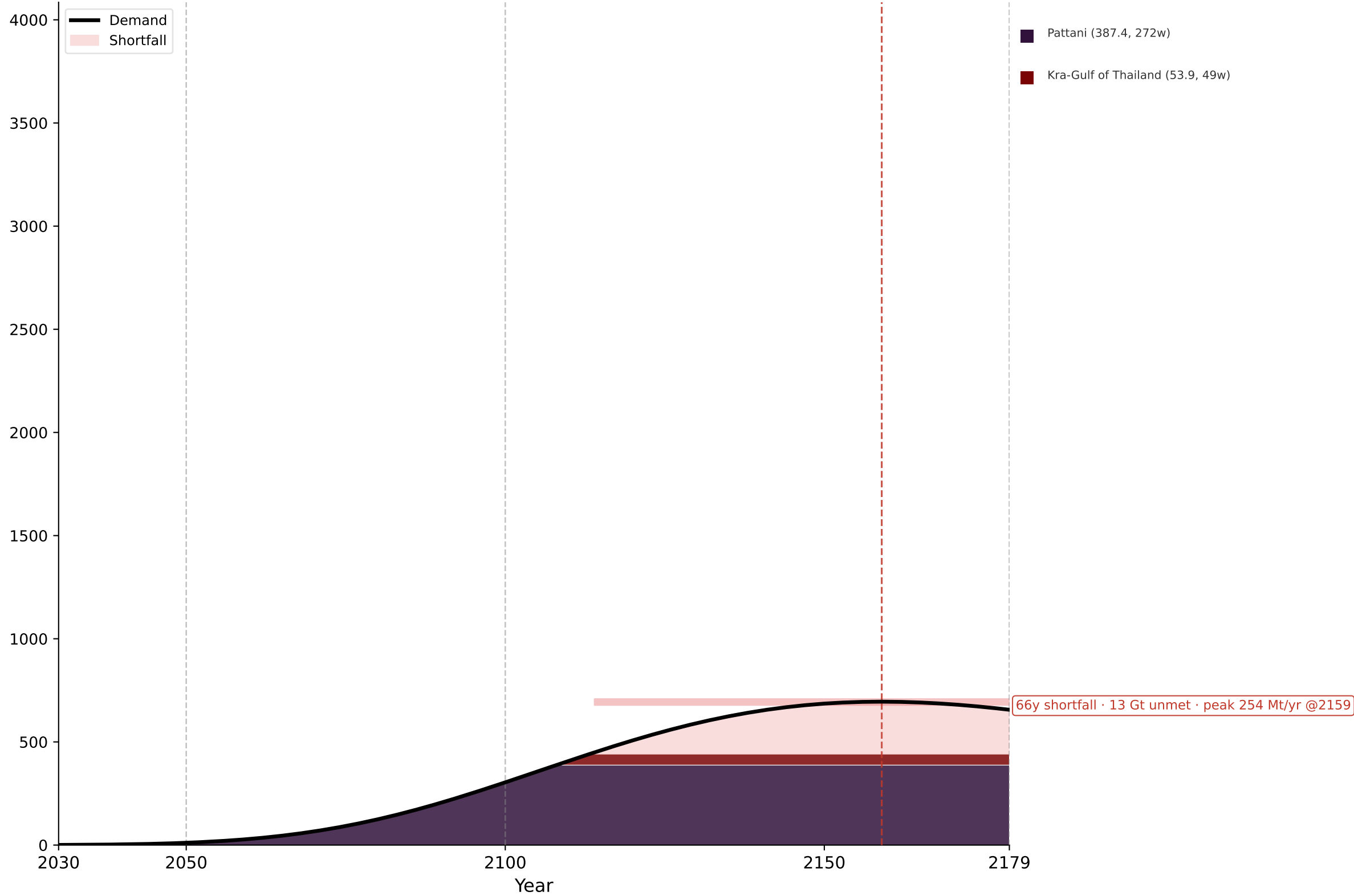
Gompertz
