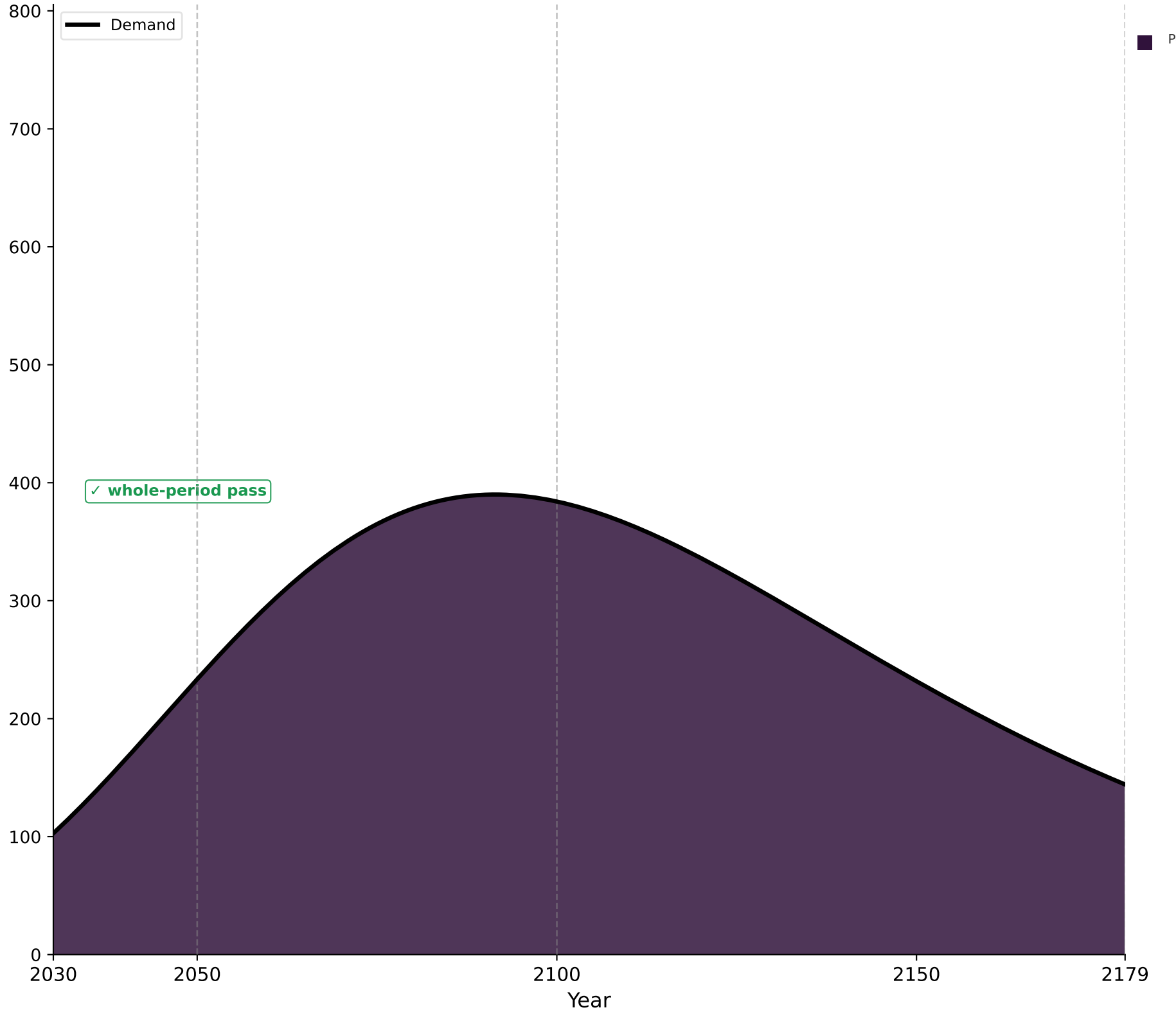
Gompertz
