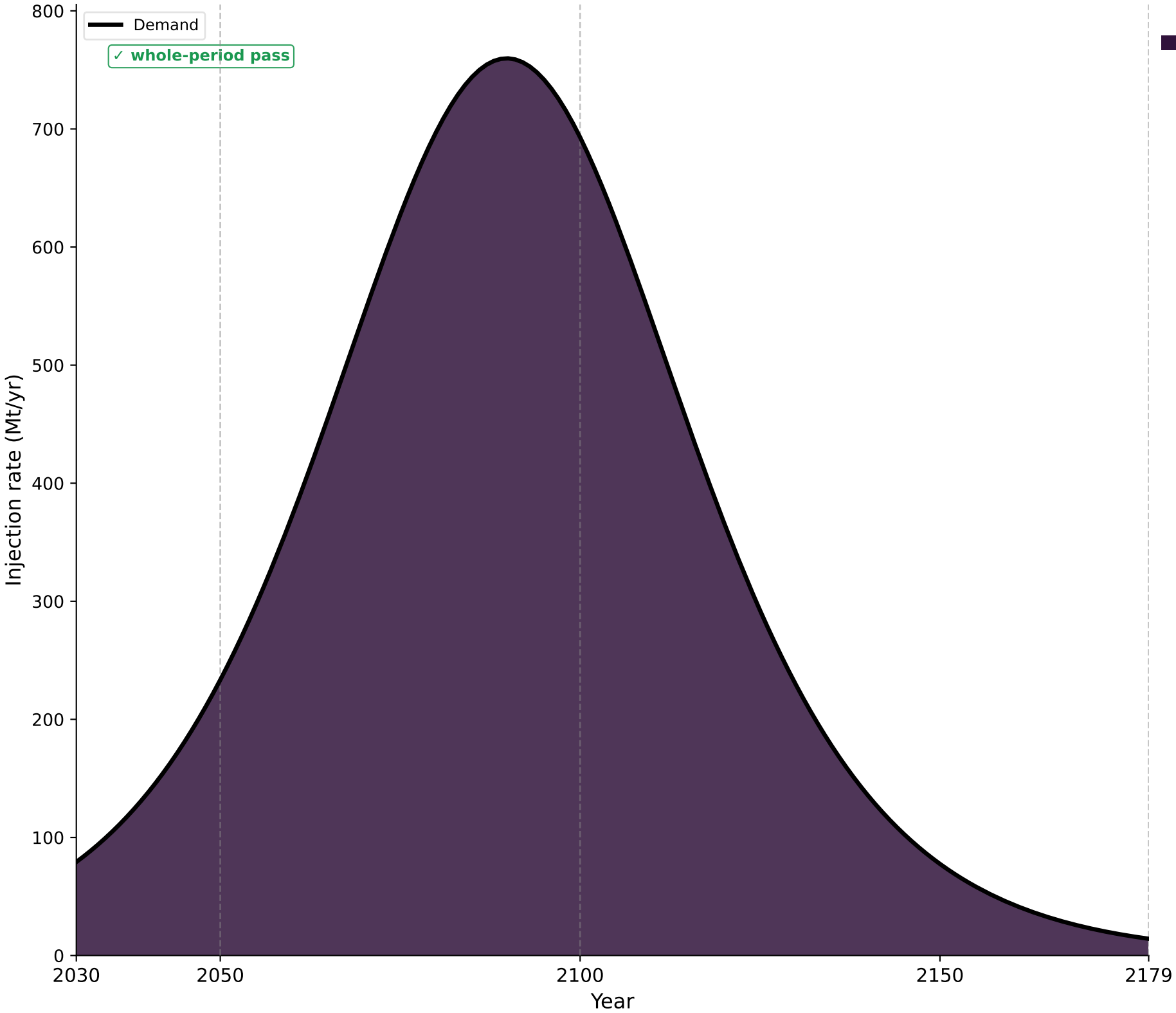
Logistic
