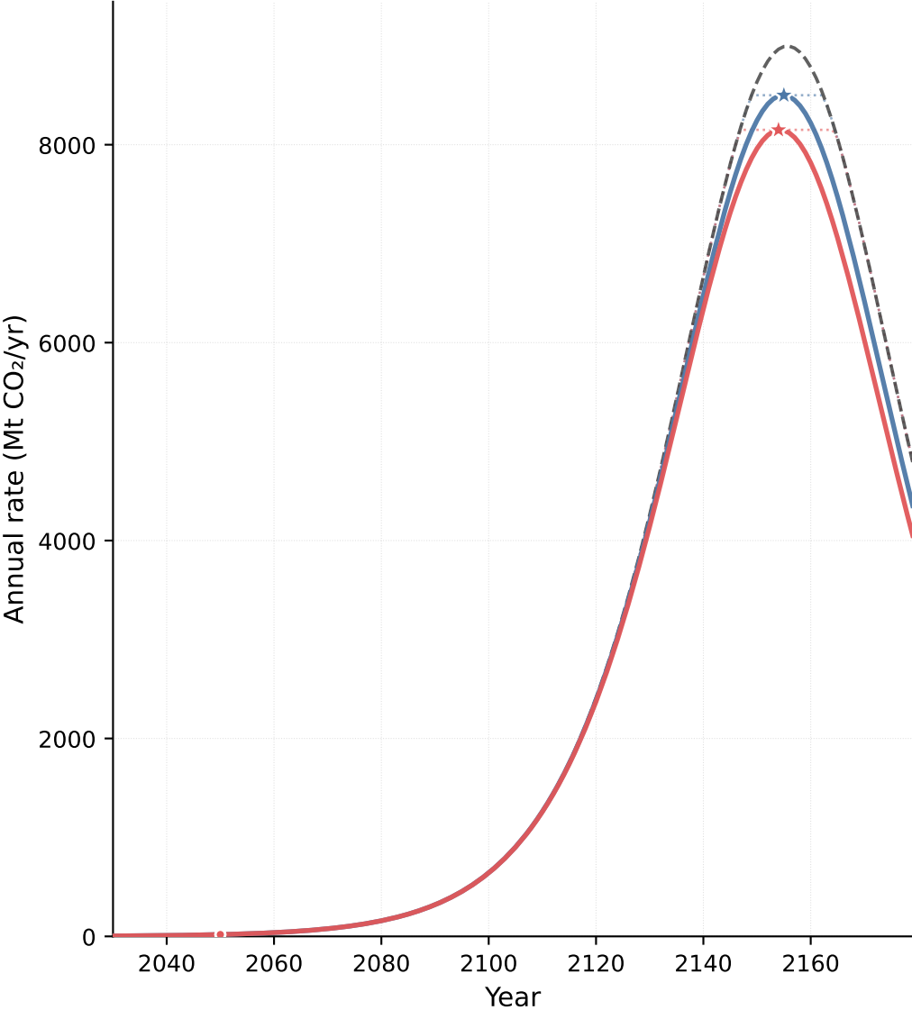
Logistic
