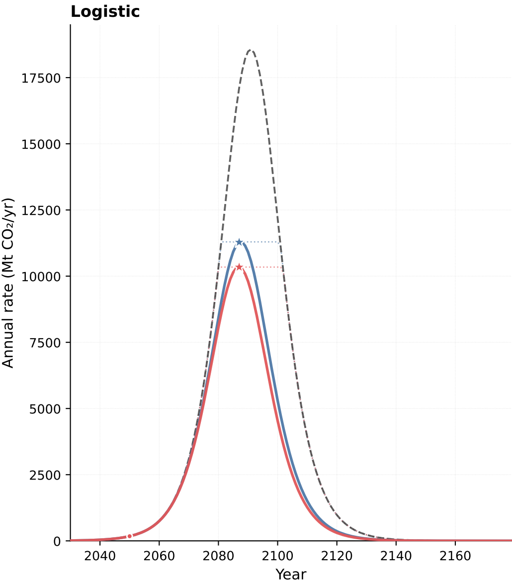
Logistic: original vs reconstructed
