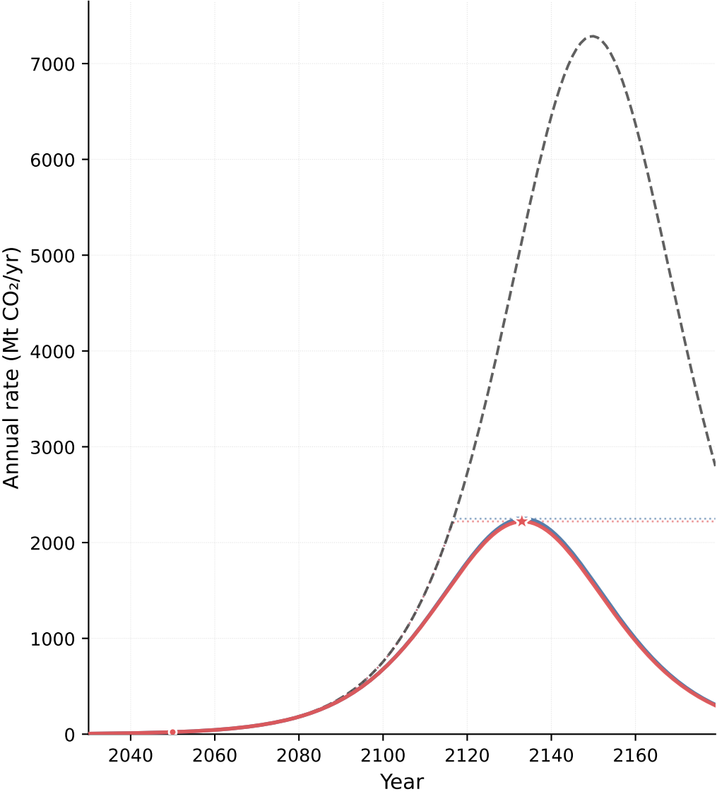
Logistic
