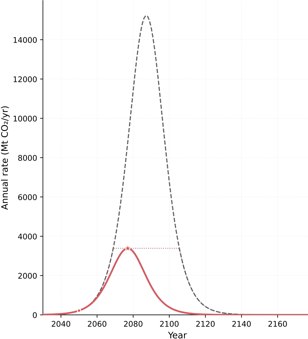
Logistic
