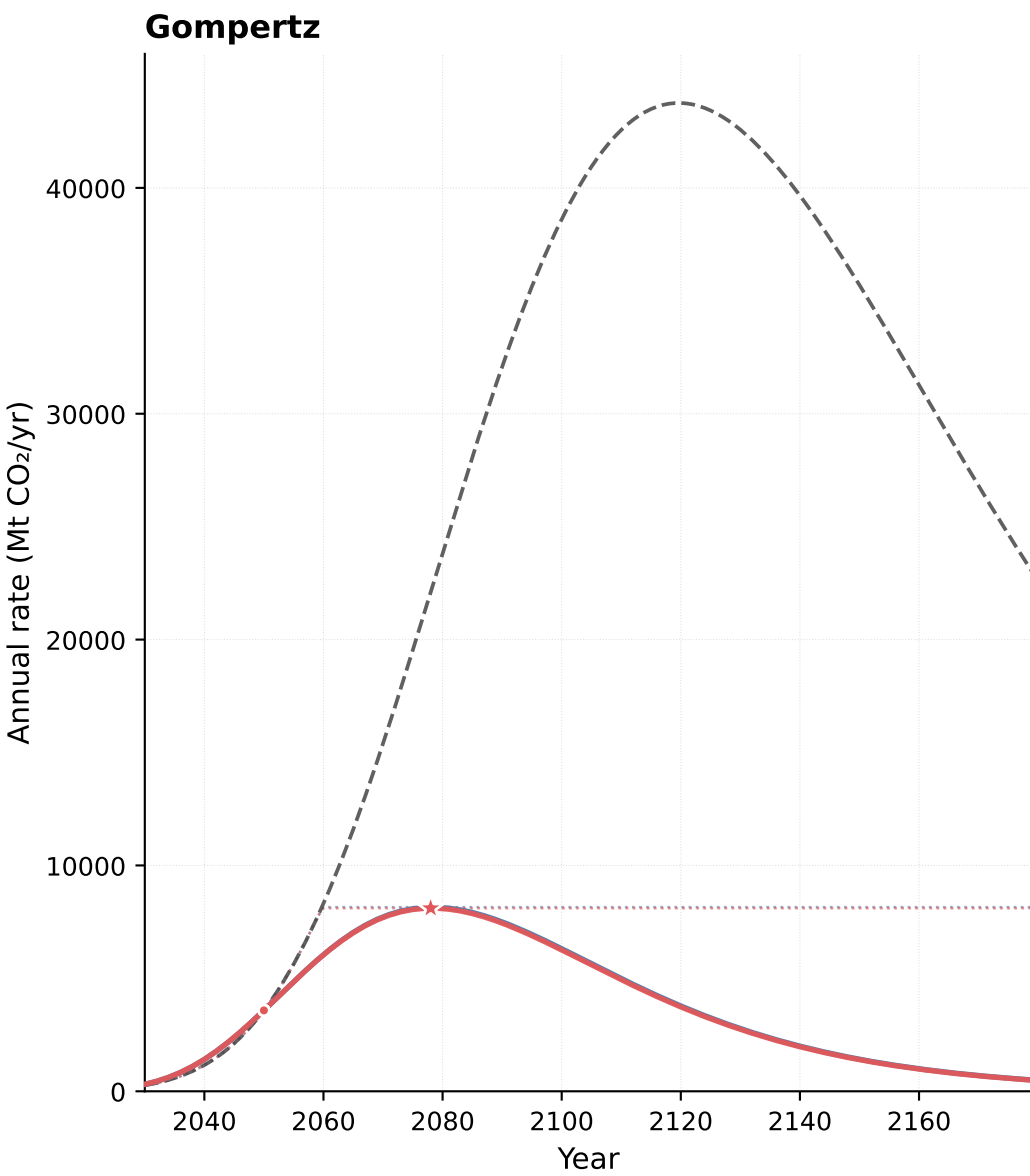
Gompertz: original vs reconstructed
