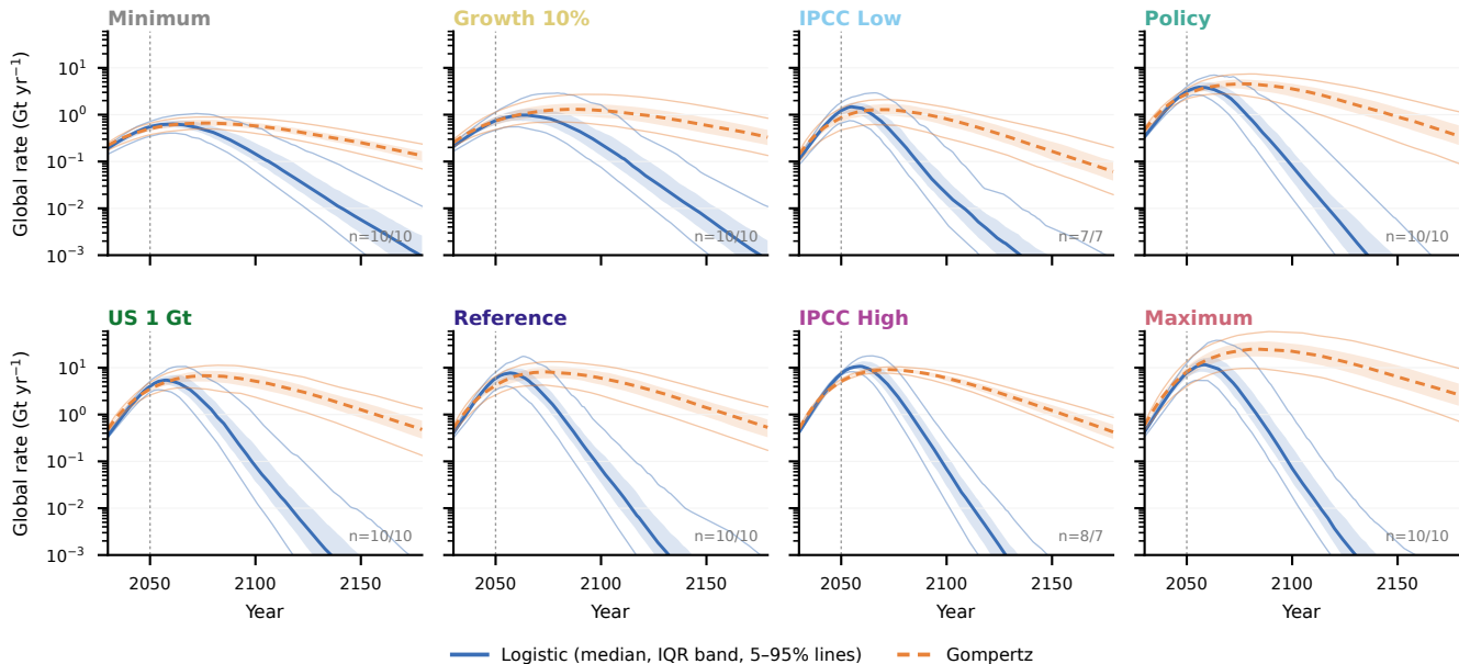
Fig. S1 | Probabilistic global storage-demand ensembles (200 Monte Carlo paths per form)
