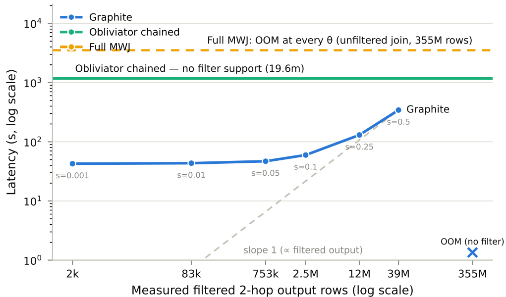
(b) Latency vs filtered output size
