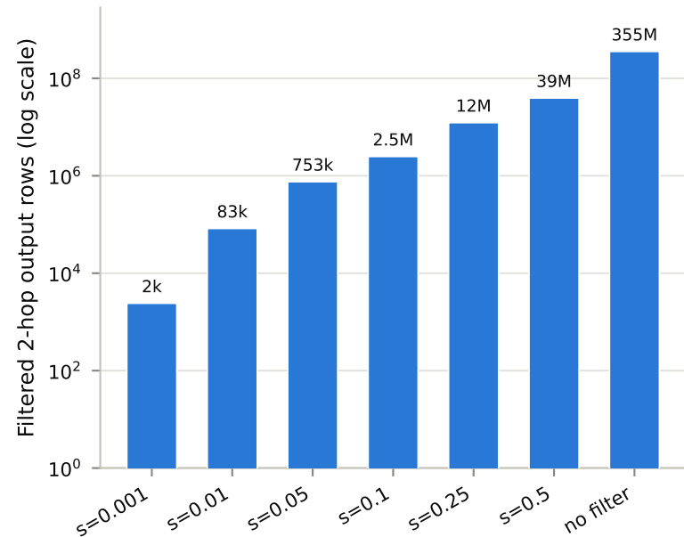
(a) Same input, predicate sweeps the output
