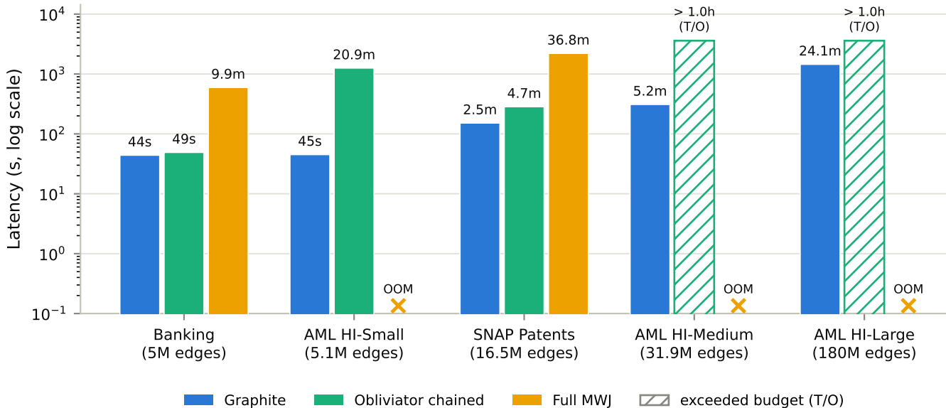
2-hop chain query across datasets
