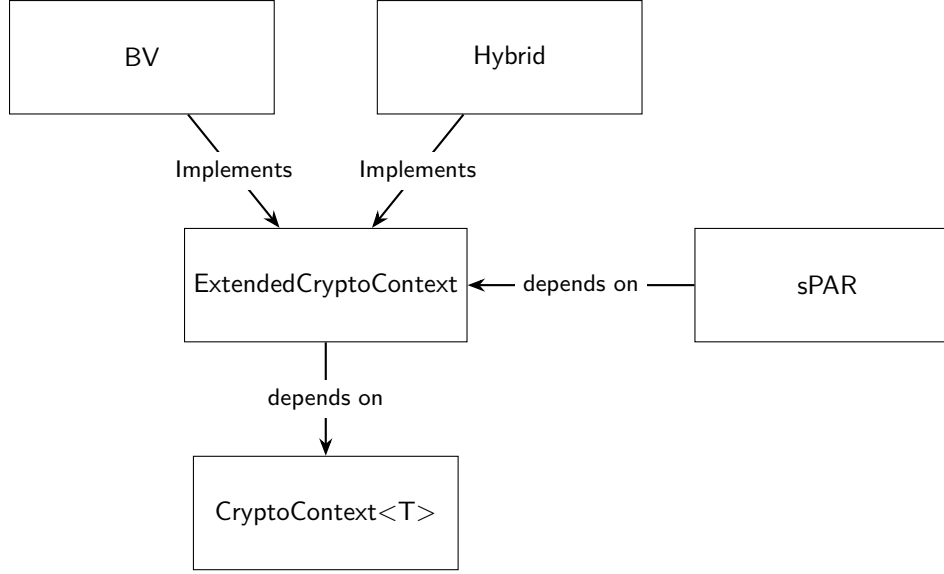
(a) Dependency graph
