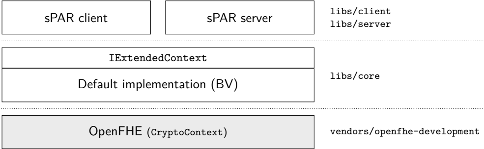
Figure 3.1: Each component depends only on what lies directly beneath it. The sPAR libraries consume the core library solely through the IExtendedContext interface.
