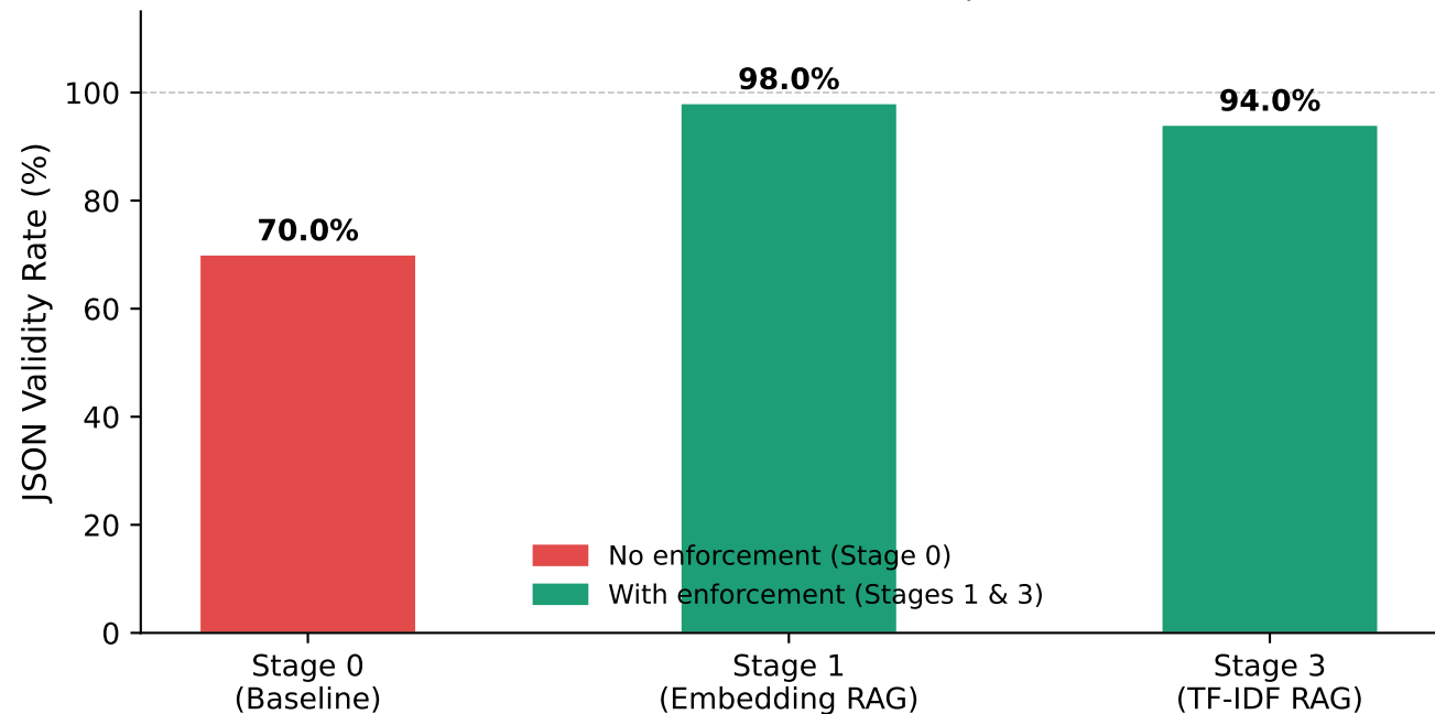
Effect of Schema Enforcement on JSON Validity (Ollama LLaMA3 8B, N=100 queries)
