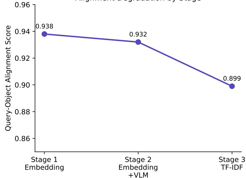
Alignment Degradation by Stage
