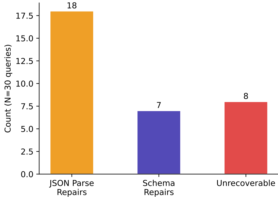
Repair Loop Activation (Complex Schema)
