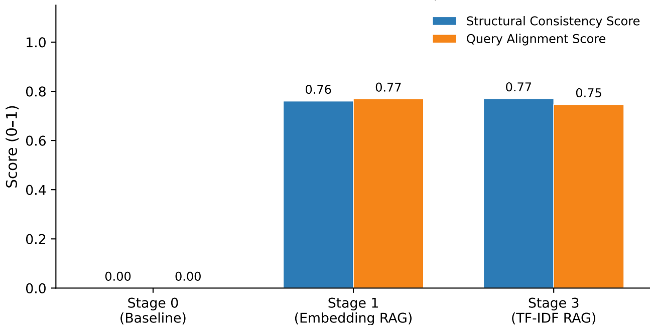
Structural Consistency & Query Alignment by Stage (Ollama LLaMA3 8B, N=100 queries)
