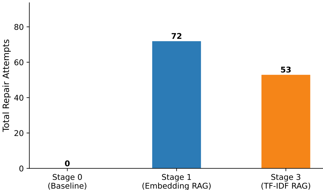
LLM Repair Attempts per Stage (Ollama LLaMA3 8B, N=100 queries)
