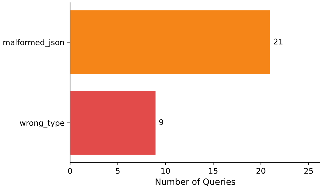
Stage 0 Failure Mode Breakdown (enforce_schema=False, N=100)
