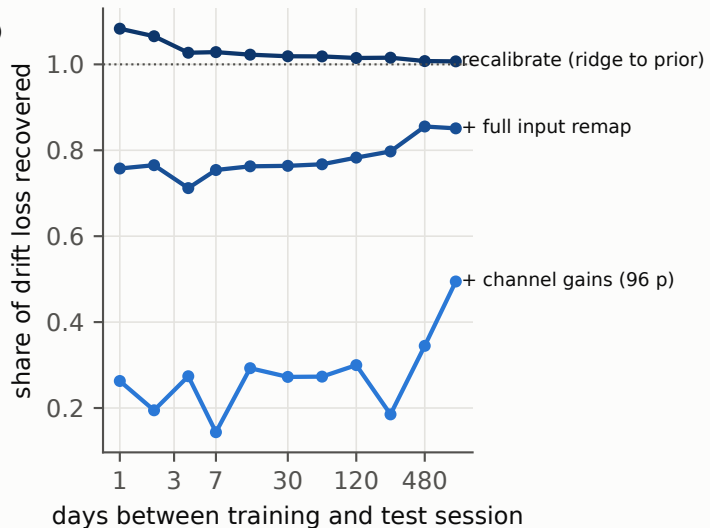
B Loss recovered beyond renormalization
