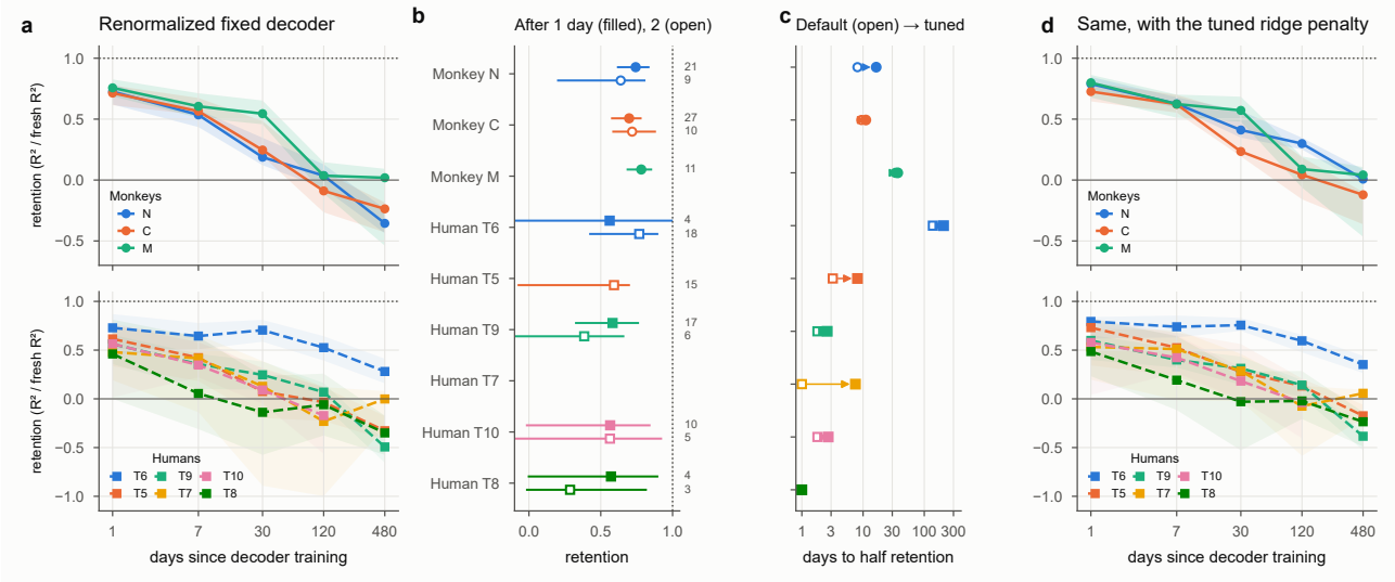
Fig. 3 Decoders decay at rates that differ between individuals. a , Retention of the renormalized fixed decoder, the R^2 of the old decoder divided by that of the reference decoder, against days since training, for monkeys (top, circles) and humans (bottom, squares). Bands show 95% confidence intervals. b , Retention after exactly one day (filled) and two days (open). Numbers give session pairs. c , Days until retention falls to one half, with the default ridge penalty (open) and the tuned penalty (filled). d , As in a , with the tuned penalty.
