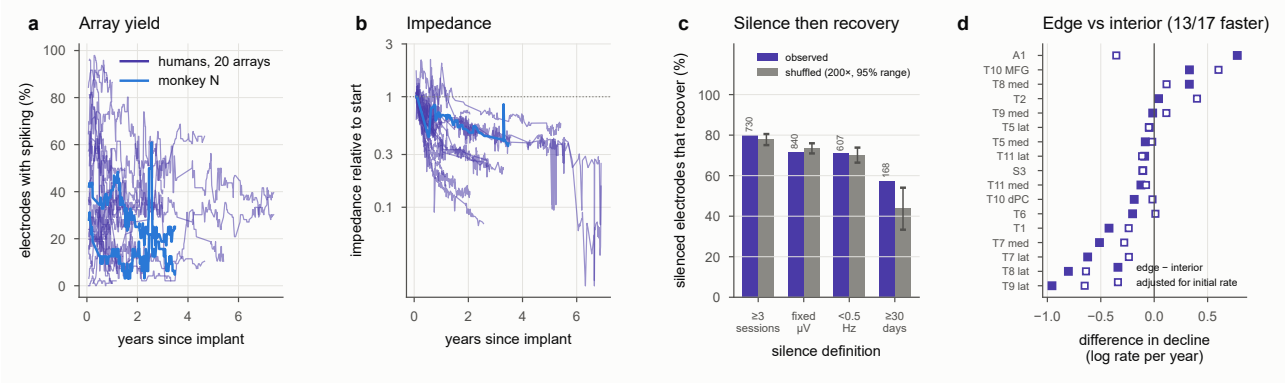
Fig. 7 Most electrode silences are transient fluctuations. a , Percentage of electrodes with spiking activity over years, for 20 human arrays (purple) and two arrays in monkey N (blue). b , Median impedance of each array relative to its first sessions. c , Percentage of silenced human electrodes that later recovered, observed (purple) and after shuffling session order 200 times (grey, with 95% range). Four definitions of silence are shown. Numbers give silenced electrodes. d , Difference in the yearly decline of firing rate between edge and interior electrodes, per human array, before (filled) and after (open) adjusting for initial firing rate.
