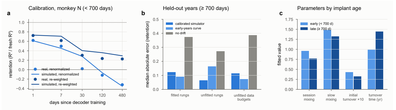
Fig. 8 A calibrated simulator for testing new corrections. a , Calibration on monkey N sessions before day 700. Points show real retention; lines show the simulator. b , Prediction error on sessions after day 700, for the simulator (dark blue), the median retention measured before day 700 (light blue) and a simulator without drift (grey). c , Parameters calibrated separately on early and late sessions.
