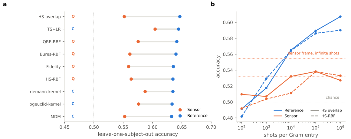
Figure 11. (a) Cross-subject transfer, leave-one-subject-out. Recentrng helps every method and helps the quantum kernels (Q) most, but in the reference frame all nine geometries are indistinguishable. (b) Accuracy against shot budget. The reference frame needs more shots to approach its own ceiling because that ceiling is higher, yet from 10^4 shots per Gram entry it already exceeds what the sensor frame attains with unlimited shots.
