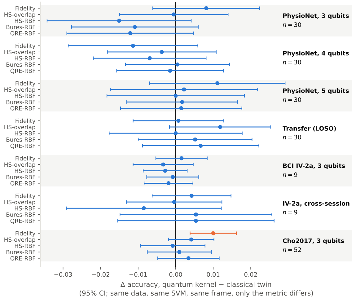
Figure 9. The decisive control. Each quantum kernel is compared against a classical SPD-manifold kernel [30] used in the same support vector machine, on the same covariances, with the same tuning budget, in the same reference frame; only the metric differs. Points are mean paired differences with 95% confidence intervals for the difference; table 9 gives the 90% intervals that correspond to the equivalence test, which are narrower. Every interval crosses zero except the fidelity kernel on Cho2017, drawn in orange, which lies inside the pre-specified margin (see text); table 12 repeats the PhysioNet block under two more partitions. Note the axis range: the entire plot spans eight accuracy points, against a frame effect (tables 7 and 11) of up to +0.217.
