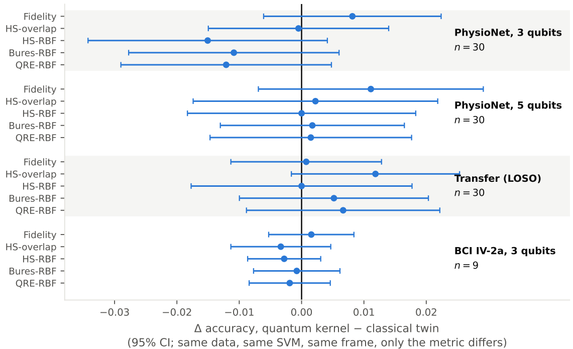
Figure 9. The decisive control. Each quantum kernel is compared against a classical SPD-manifold kernel [29] used in the same support vector machine, on the same covariances, with the same tuning budget, in the same reference frame; only the metric differs. Points are mean paired differences with 95% confidence intervals for the difference; table 9 gives the 90% intervals that correspond to the equivalence test, which are narrower. Every interval here crosses zero in all four settings. Note the axis range: the entire plot spans eight accuracy points, against a frame effect (figure 8) of up to nineteen.
