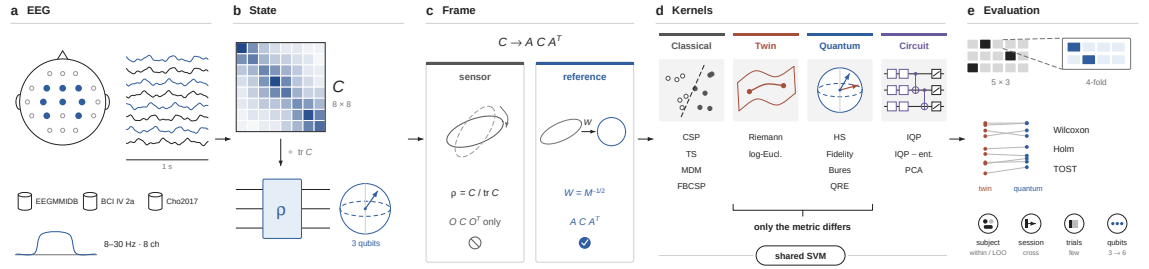
Figure 2. Study design, and where the control sits. (a) Three public motor-imagery datasets, PhysioNet EEGMMIDB (104 subjects, 45 trials), BCI Competition IV-2a (9 subjects, 288 trials, two sessions) and Cho2017 (52 subjects), reduced to the same eight sensorimotor electrodes, the same 8–30 Hz band and the same one-second window, so every difference reported here is a property of the method and not of the preprocessing. (b) Each trial becomes an 8 \times 8 spatial covariance matrix C ; divided by its trace it is a density matrix \rho on \log_2 8 = 3 qubits, with no dimensional reduction and no angle embedding. (c) EEG’s nuisances (electrode gain, head geometry, skull conductivity, source mixing) act by congruence C \mapsto A C A^\top . The density-matrix kernels are invariant only under the orthogonal subgroup in the sensor frame, and exactly invariant under the full group in the reference frame of (6), where W = M^{-1/2} and the Fréchet mean M is estimated label-free from training trials alone. Every suite is run in both frames. (d) Four pipeline families under one protocol. The bracket marks the paper’s central control: the classical Riemannian twin and the quantum kernels consume the same covariances, sit in the same support vector machine, receive the same tuning budget and are expressed in the same frame, so the only thing that differs between them is the metric. (e) Nested cross-validation (5 folds \times 3 repeats outer, 4-fold inner, identical budget for every pipeline), paired per-subject Wilcoxon signed-rank with Holm correction inside each pre-specified family, and two one-sided tests for equivalence against the twin, across the five evaluation settings.
