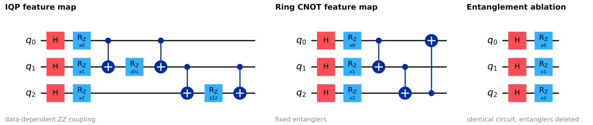
Figure 4. The circuit feature maps, at three qubits with one layer shown. Rotation angles carry the PCA-reduced tangent-space features and the kernel is the state overlap |\langle \phi(x) | \phi(z) \rangle|^2 . The IQP map uses data-dependent ZZ couplings; the ring map uses fixed CNOTs. The third panel is the entanglement ablation: the identical circuit with every entangling gate deleted, which factorises the kernel into single-qubit terms and isolates what entanglement contributes. The figure is rendered by Qiskit from a circuit that is checked against the executed PennyLane circuit before drawing: the two agree on full Gram matrices to < 10^{-15} , so the diagram cannot drift from the code it documents.
