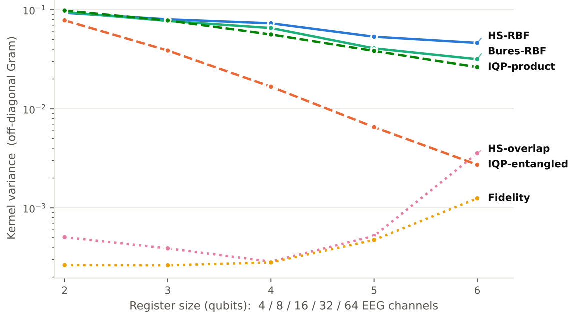
Figure 5. Kernel variance versus register size on real EEG ( n = 10 subjects). Lower is worse: a kernel whose variance collapses cannot separate trials. Line style encodes the kernel family. The entangled circuit kernel (orange, dashed) decays fastest.
