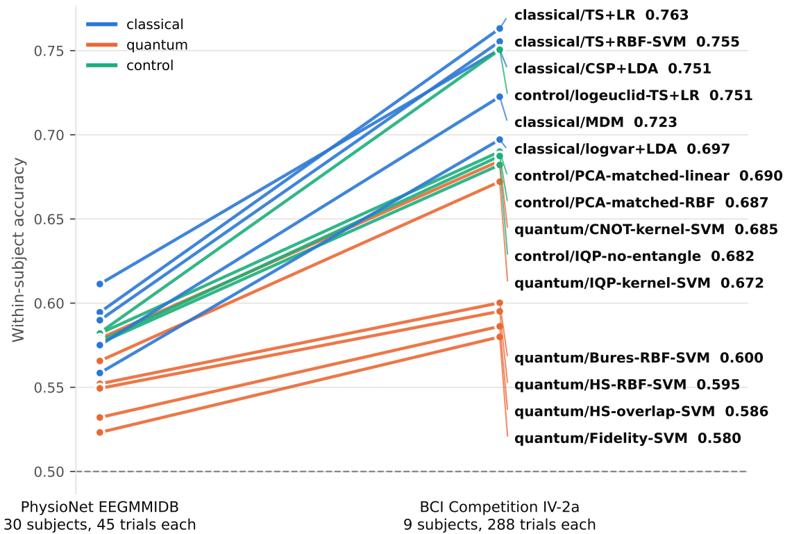
Figure 6. The same 15 pipelines on two datasets at opposite corners of the design space. Identical channels, protocol, tuning budget and code; only the data differs. Line slope is the quantity of interest: classical and control pipelines rise steeply with the extra trials while the four density-matrix and overlap kernels stay low. The dashed line marks chance.
