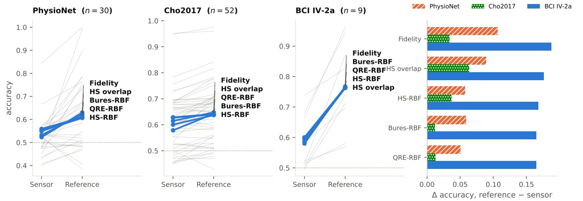
Figure 7. Accuracy in the sensor frame versus the reference frame. Thin lines are individual subjects, shown for the Fidelity kernel only. Every kernel improves on all three datasets; on IV-2a every kernel improves in every subject. The correction is worth two to three times more on IV-2a than on PhysioNet, and least on Cho2017, whose sensor-frame kernels start closest to the classical baselines.
