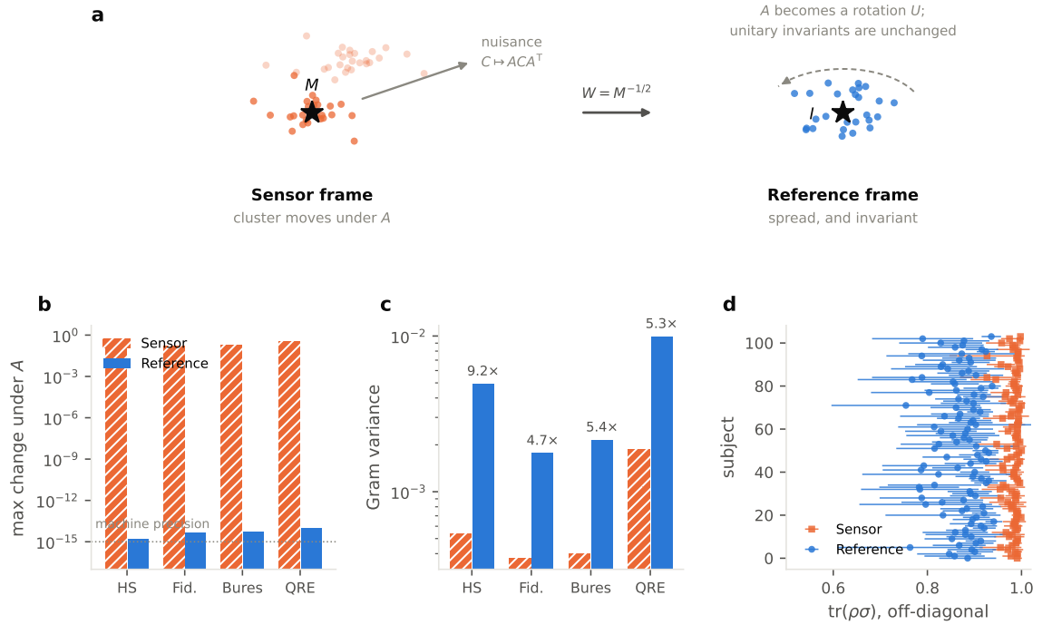
Figure 3. (a) EEG covariances cluster tightly about their Fréchet mean M , and a nuisance congruence moves the whole cluster. Whitening by M spreads the states about the identity and reduces the nuisance to a common rotation, to which every quantum invariant is blind. (b) The proposition verified numerically: reference-frame residuals sit at machine precision, sensor-frame ones are O(10^{-1}) . (c) Off-diagonal Gram variance rises by 4.7–9.2 \times in the reference frame. (d) The sensor-frame overlaps saturate near unity in every subject ( n = 104 ).
