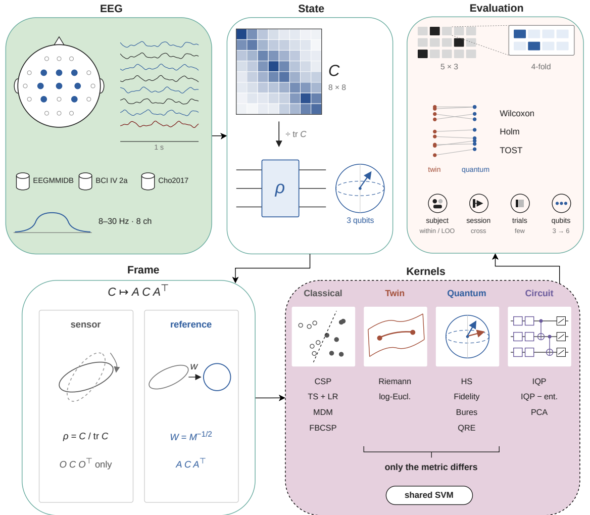
Figure 2. Study design, and where the control sits. Arrows give the order of processing: EEG to State to Frame to Kernels to Evaluation. EEG : three public motor-imagery datasets, PhysioNet EEGMMIDB (104 subjects, 45 trials), BCI Competition IV-2a (9 subjects, 288 trials, two sessions) and Cho2017 (52 subjects), reduced to the same eight sensorimotor electrodes (filled), the same 8–30 Hz band and the same one-second window, so every difference reported here is a property of the method and not of the preprocessing. State : each trial becomes an 8 \times 8 spatial covariance C ; divided by its trace it is a density matrix \rho on \log_2 8 = 3 qubits, with no dimensionality reduction and no angle embedding. Frame : EEG’s nuisances (electrode gain, head geometry, skull conductivity, source mixing) act by congruence C \mapsto ACA^T . The density-matrix kernels are invariant only under the orthogonal subgroup in the sensor frame, and exactly invariant under the full group in the reference frame of (6), where W = M^{-1/2} and the Fréchet mean M is estimated label-free from training trials alone. Every suite is run in both frames. Kernels : four pipeline families under one protocol. The bracket marks the paper’s central control: the classical Riemannian twin and the quantum kernels consume the same covariances, sit in the same support vector machine, receive the same tuning budget and are expressed in the same frame, so the only thing that differs between them is the metric. Evaluation : nested cross-validation (5 folds \times 3 repeats outer, 4-fold inner, identical budget for every pipeline), paired per-subject Wilcoxon signed-rank with Holm correction inside each pre-specified family, and two one-sided tests for equivalence against the twin, across the five evaluation settings. The editable source of this figure is distributed with the manuscript as architecture.drawio .
