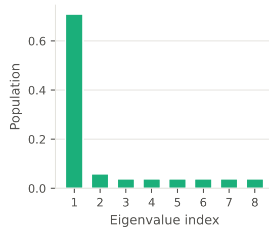
(e) Spectrum of \rho , sums to 1
