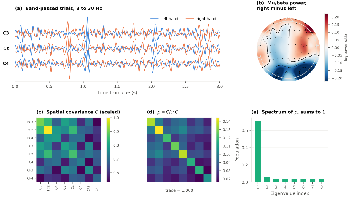
Figure 1. From scalp EEG to a quantum state, computed from real recordings rather than simulated. (a) Band-passed sensorimotor traces for one left-hand and one right-hand trial. (b) Scalp topography of mu/beta power, right minus left: power falls over the hemisphere contralateral to the imagined hand, which is the physiological effect every decoder in this study exploits. (c) The spatial covariance of a single trial over the eight decoding channels. (d) The same matrix divided by its trace. It is now a density matrix, and (e) its eigenvalues are non-negative and sum to one, so they are a population distribution. The step from (c) to (d) is the whole encoding: no dimensionality reduction, no rotation-angle embedding.
