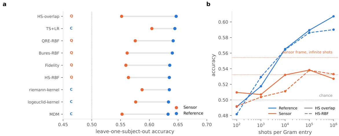
Figure 10. (a) Cross-subject transfer, leave-one-subject-out. Recentring helps every method and helps the quantum kernels (Q) most, but in the reference frame all nine geometries are indistinguishable. (b) Accuracy against shot budget. The reference frame needs more shots to approach its own ceiling because that ceiling is higher, yet from 10^4 shots per Gram entry it already exceeds what the sensor frame attains with unlimited shots.
