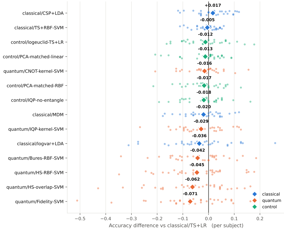
Figure 5. Paired per-subject accuracy differences against the Riemannian tangent-space reference. Dots are individual subjects; diamonds are means. Points left of zero indicate worse performance than the reference.
