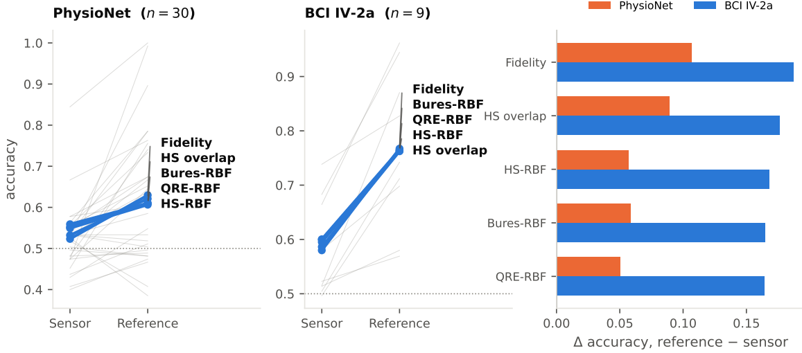
Figure 8. Accuracy in the sensor frame versus the reference frame. Thin lines are individual subjects, shown for the Fidelity kernel only. Every kernel improves on both datasets; on IV-2a every kernel improves in every subject. The correction is worth two to three times more on IV-2a, where the reference state is estimated from 288 rather than 45 trials per subject.
