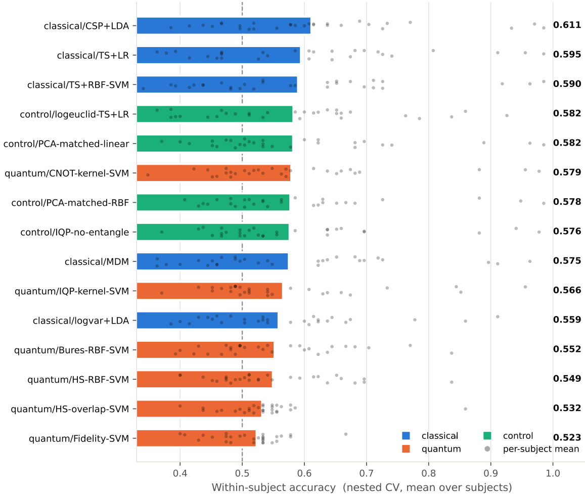
Figure 4. Within-subject accuracy by pipeline ( n = 30 subjects, nested cross-validation). Bars are means over subjects; grey dots are individual subject means. The dashed line marks chance. Every pipeline, classical baselines included, received the same inner hyperparameter search.
