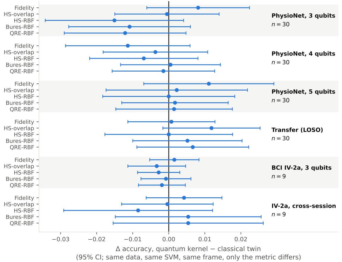
Figure 9. The decisive control. Each quantum kernel is compared against a classical SPD-manifold kernel [29] used in the same support vector machine, on the same covariances, with the same tuning budget, in the same reference frame; only the metric differs. Points are mean paired differences with 95% confidence intervals for the difference; table 9 gives the 90% intervals that correspond to the equivalence test, which are narrower. Every interval here crosses zero in all six settings at the primary partition (table 12 for two more). Note the axis range: the entire plot spans eight accuracy points, against a frame effect (tables 7 and 11) of up to +0.217.
