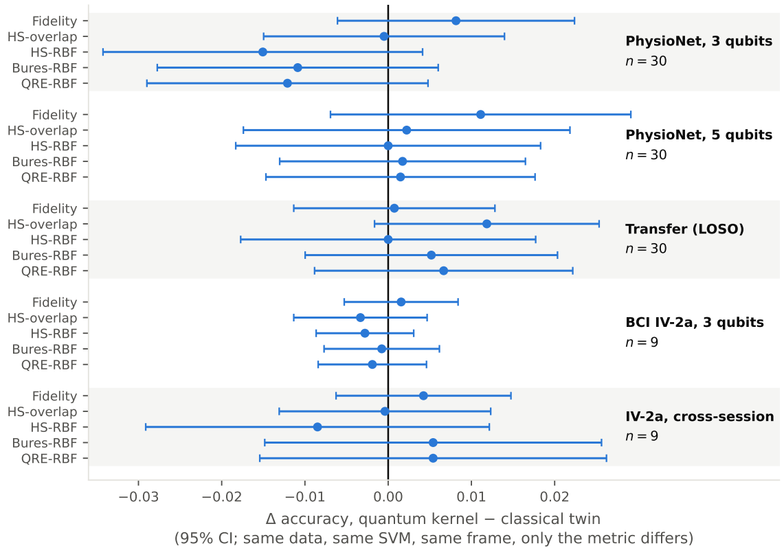
Figure 9. The decisive control. Each quantum kernel is compared against a classical SPD-manifold kernel [29] used in the same support vector machine, on the same covariances, with the same tuning budget, in the same reference frame; only the metric differs. Points are mean paired differences with 95% confidence intervals for the difference; table 9 gives the 90% intervals that correspond to the equivalence test, which are narrower. Every interval here crosses zero in all five settings. Note the axis range: the entire plot spans eight accuracy points, against a frame effect (tables 7 and 11) of up to +0.217.
