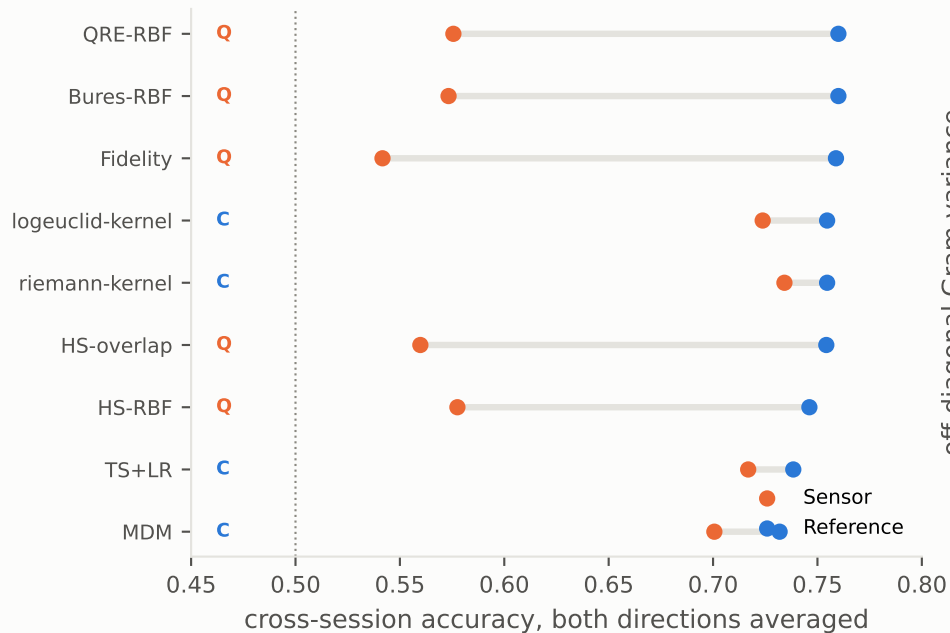
(a) Cross-session transfer on IV-2a: in the sensor frame the quantum kernels sit near chance while the classical baselines do not; recentring each session by its own label-free mean closes the gap and leaves every geometry tied.
