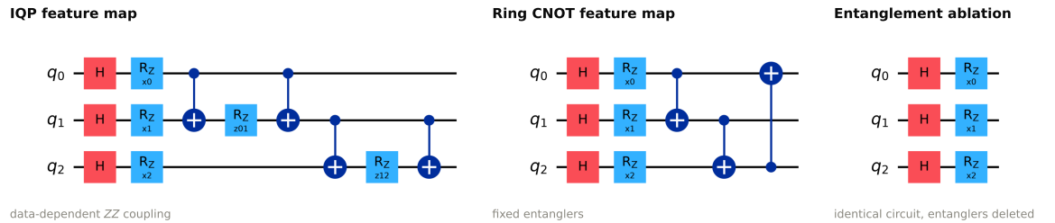
Figure 5. The circuit feature maps, at three qubits with one layer shown. Rotation angles carry the PCA-reduced tangent-space features and the kernel is the state overlap |\langle\phi(x)|\phi(z)\rangle|^2 . The IQP map uses data-dependent ZZ couplings; the ring map uses fixed CNOTs. The third panel is the entanglement ablation: the identical circuit with every entangling gate deleted, which factorises the kernel into single-qubit terms and isolates what entanglement contributes. The figure is rendered by Qiskit from a circuit that is checked against the executed PennyLane circuit before drawing: the two agree on full Gram matrices to < 10^{-15} , so the diagram cannot drift from the code it documents.
