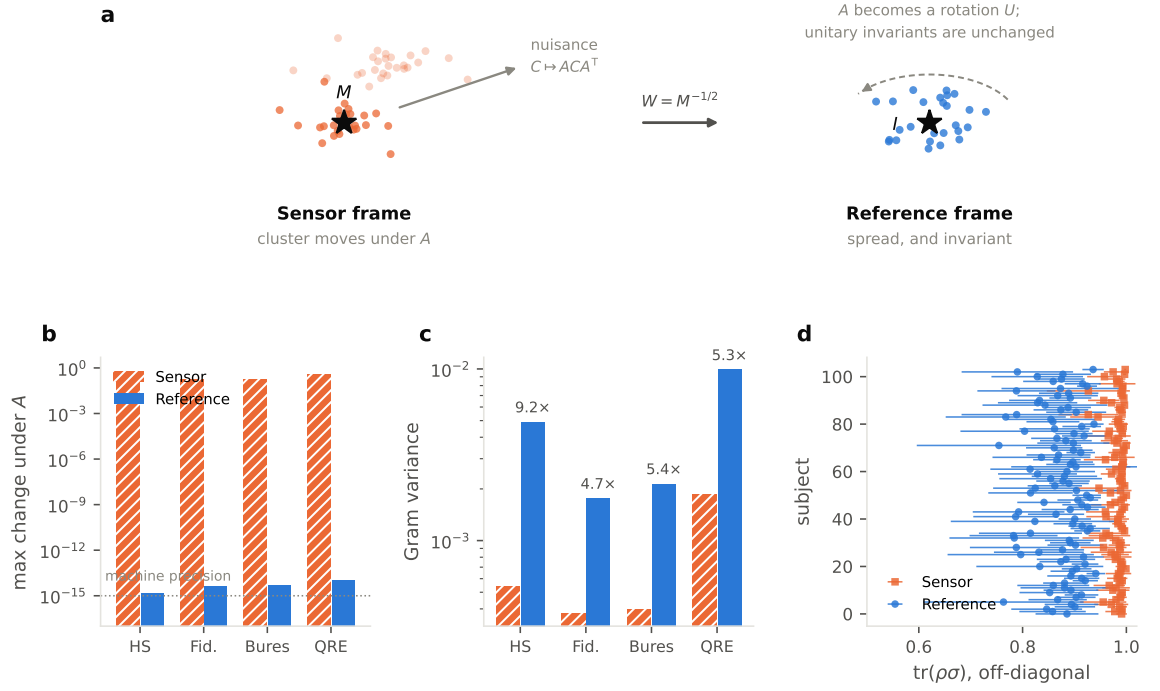
Figure 4. (a) EEG covariances cluster tightly about their Fréchet mean M , and a nuisance congruence moves the whole cluster. Whitening by M spreads the states about the identity and reduces the nuisance to a common rotation, to which every quantum invariant is blind. (b) The proposition verified numerically: reference-frame residuals sit at machine precision, sensor-frame ones are O(10^{-1}) . (c) Off-diagonal Gram variance rises by 4.7–9.2 \times in the reference frame. (d) The sensor-frame overlaps saturate near unity in every subject ( n = 104 ).
