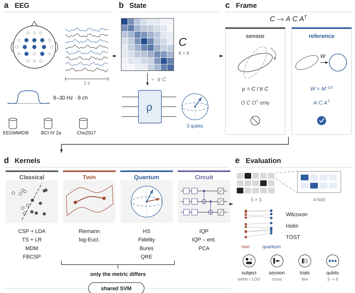
Figure 2. Study design, and where the control sits. (a) Three public motor-imagery datasets, PhysioNet EEGMMIDB (104 subjects, 45 trials), BCI Competition IV-2a (9 subjects, 288 trials, two sessions) and Cho2017 (52 subjects), reduced to the same eight sensorimotor electrodes, the same 8–30 Hz band and the same one-second window, so every difference reported here is a property of the method and not of the preprocessing. (b) Each trial becomes an 8 \times 8 spatial covariance C ; divided by its trace it is a density matrix \rho on \log_2 8 = 3 qubits, with no dimensionality reduction and no angle embedding. (c) EEG’s nuisances (electrode gain, head geometry, skull conductivity, source mixing) act by congruence C \mapsto A C A^T . The density-matrix kernels are invariant only under the orthogonal subgroup in the sensor frame, and exactly invariant under the full group in the reference frame of (6), where W = M^{-1/2} and the Fréchet mean M is estimated label-free from training trials alone. Every suite is run in both frames. (d) Four pipeline families under one protocol. The bracket marks the paper’s central control: the classical Riemannian twin and the quantum kernels consume the same covariances, sit in the same support vector machine, receive the same tuning budget and are expressed in the same frame, so the only thing that differs between them is the metric. (e) Nested cross-validation (5 folds \times 3 repeats outer, 4-fold inner, identical budget for every pipeline), paired per-subject Wilcoxon signed-rank with Holm correction inside each pre-specified family, and two one-sided tests for equivalence against the twin, across the five evaluation settings.
