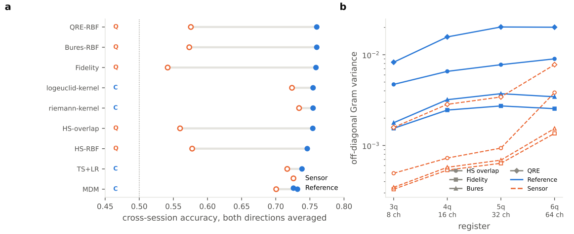
Figure 10. (a) Cross-session transfer within subject on IV-2a, both directions averaged. In the sensor frame the quantum kernels sit near chance while the classical baselines do not; whitening each session by its own label-free mean closes the gap and leaves every SPD-kernel geometry tied. (b) Off-diagonal Gram variance versus register size in both frames on PhysioNet ( n = 14 ). Solid, reference frame; dashed, sensor frame. In the reference frame no kernel falls below its three-qubit value at any larger register.
