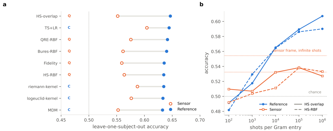
Figure 11. (a) Cross-subject transfer, leave-one-subject-out. Recentring helps every method and helps the quantum kernels (Q) most, but in the reference frame all nine geometries are indistinguishable. (b) Accuracy against shot budget. The reference frame needs more shots to approach its own ceiling because that ceiling is higher, yet from 10^4 shots per Gram entry it already exceeds what the sensor frame attains with unlimited shots.
