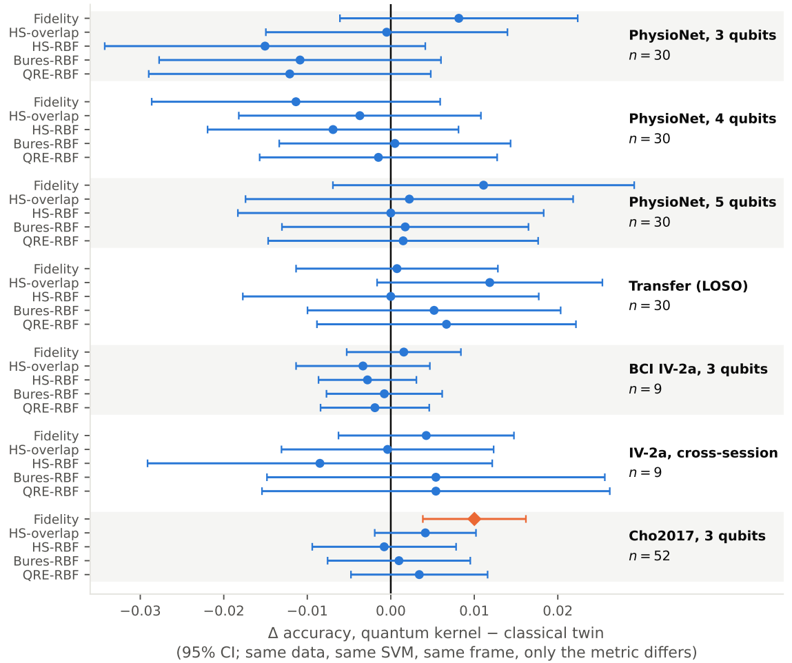
Figure 9. The decisive control. Each quantum kernel is compared against a classical SPD-manifold kernel [31] used in the same support vector machine, on the same covariances, with the same tuning budget, in the same reference frame; only the metric differs. Points are mean paired differences with 95% confidence intervals for the difference; table 9 gives the 90% intervals that correspond to the equivalence test, which are narrower. Every interval crosses zero except the fidelity kernel on Cho2017, drawn as an orange diamond, which lies inside the pre-specified margin (see text); table 12 repeats the PhysioNet block under two more partitions. Note the axis range: the entire plot spans eight accuracy points, against a frame effect (tables 7 and 11) of up to +0.217.
