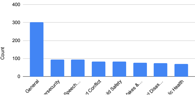
Category breakdown
