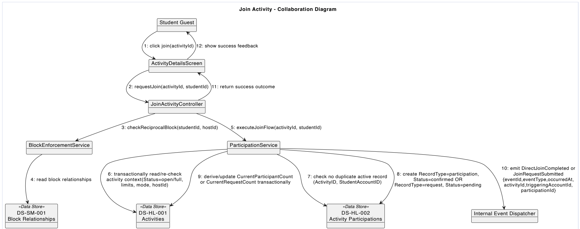
Figure 6.12: Original collaboration diagram - Join Activity.
