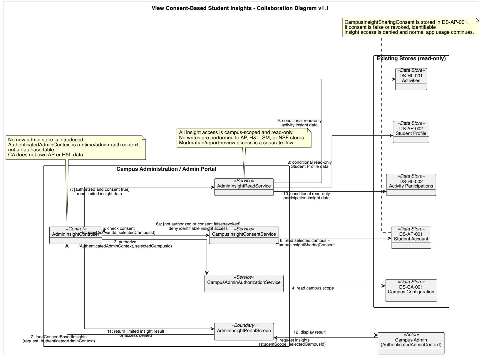
Figure 6.18: Original collaboration diagram - Consent-Based Student Insights.
