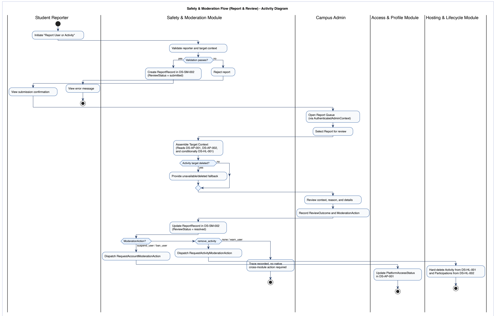
Appendix Figure H.9: Safety and Moderation Flow.
