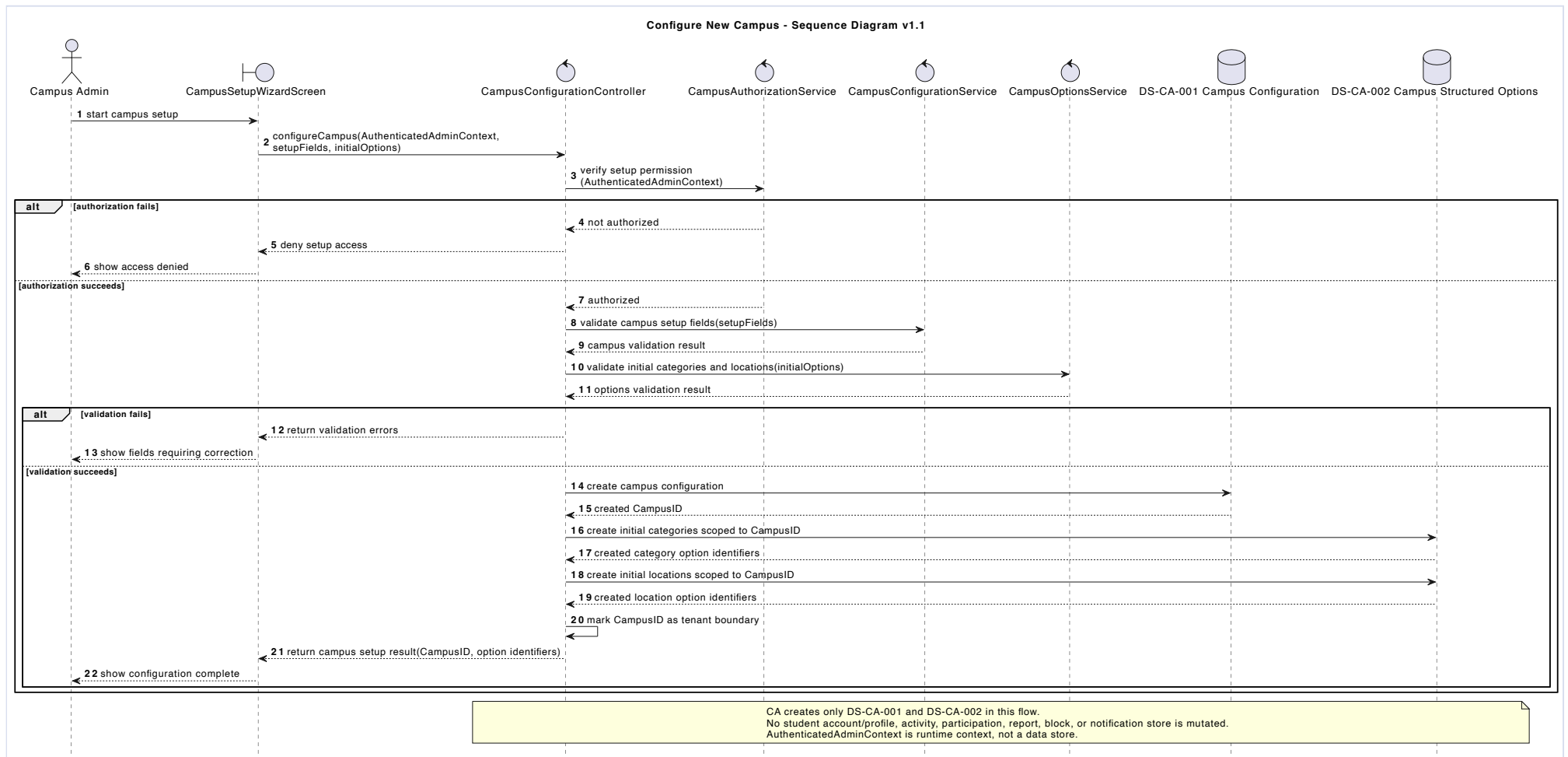
Appendix Figure H.15: Configure New Campus Sequence Diagram.
