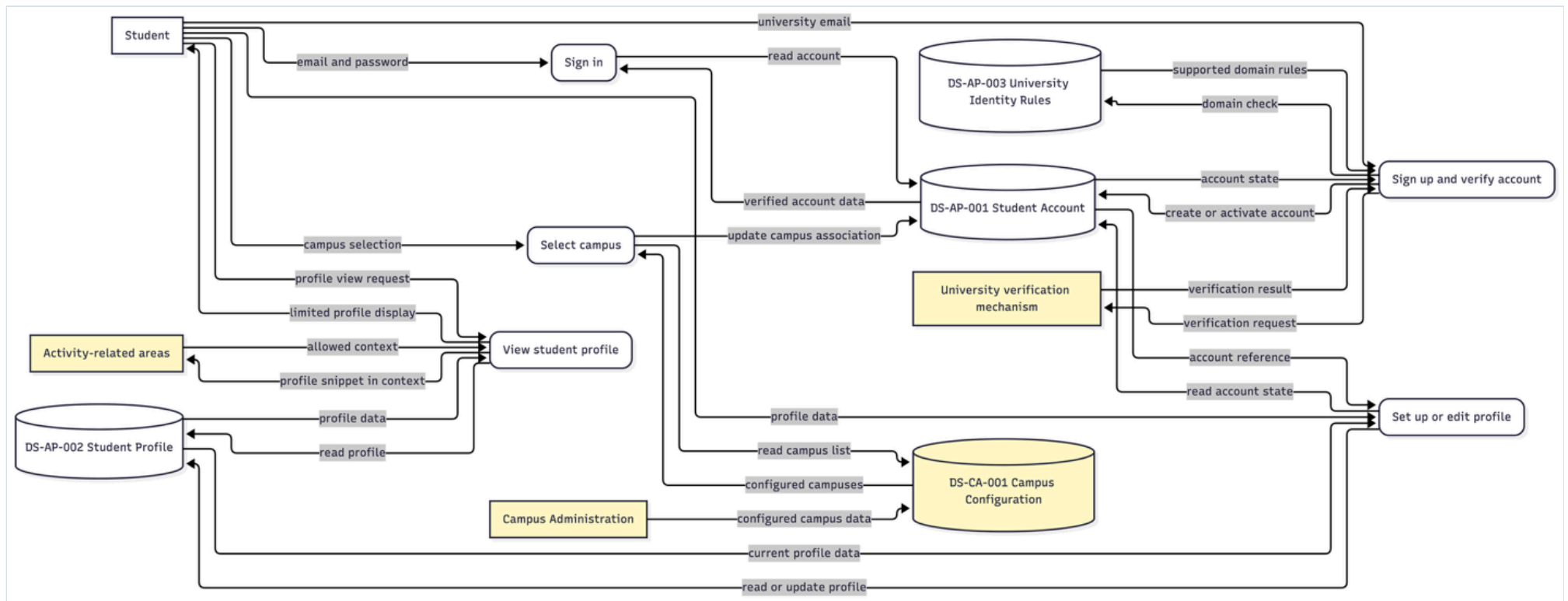
Figure 4.2: Original requirements-report subgroup DFD example recovered from the DOCX media package.
