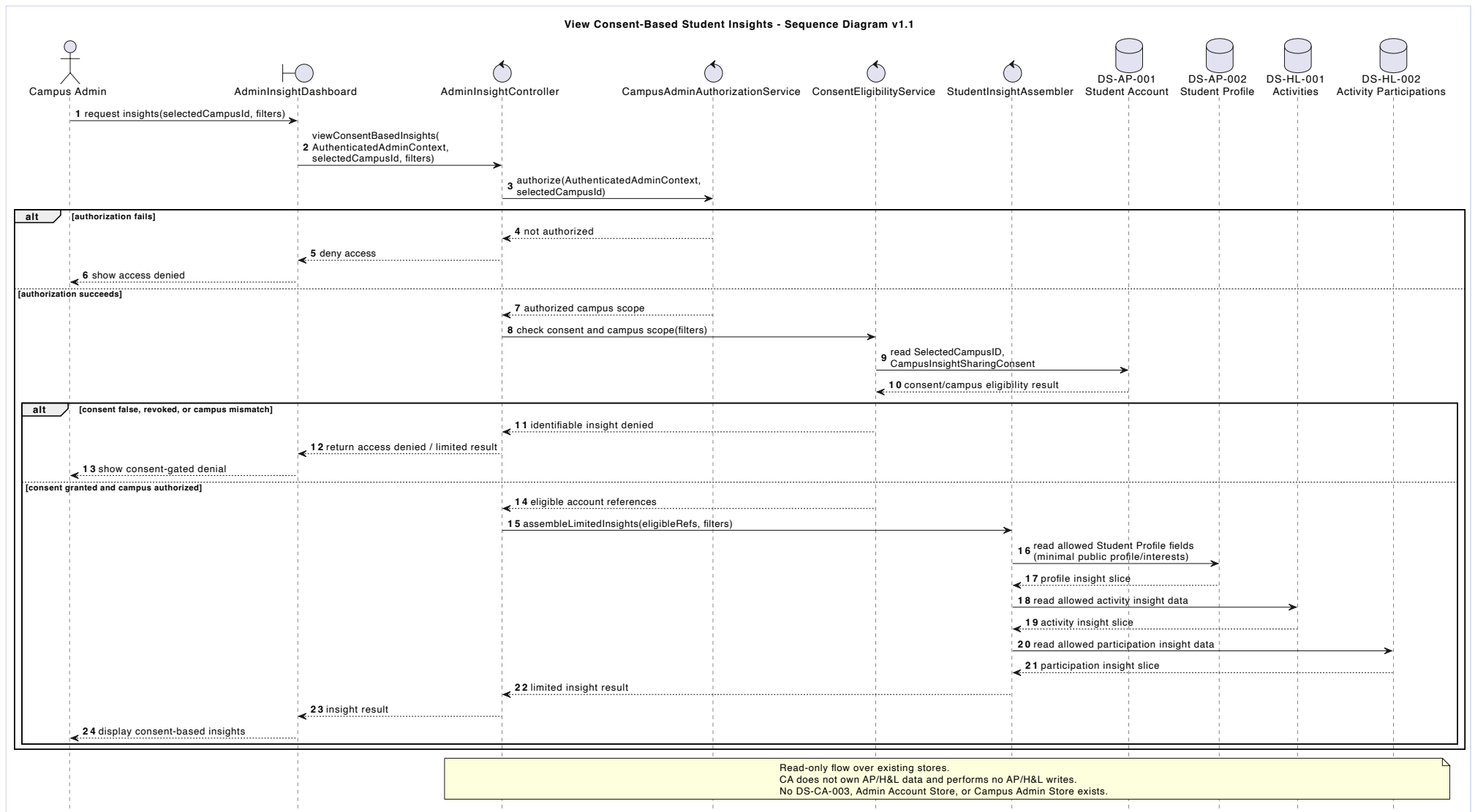
Figure 6.11: Original sequence diagram - View Consent-Based Student Insights.
