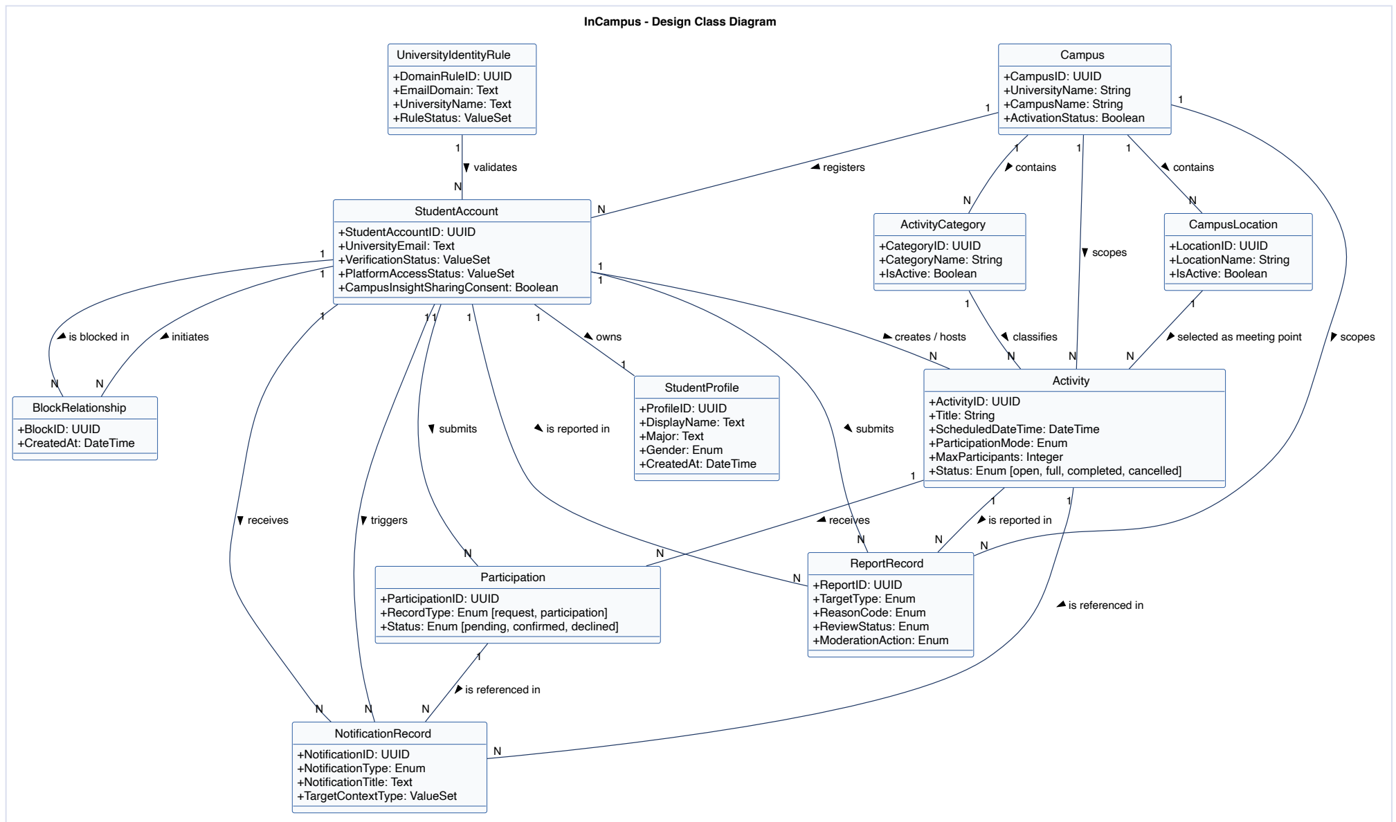
Figure 6.2: Original design class diagram recovered from the Object-Oriented Design Report DOCX media.
