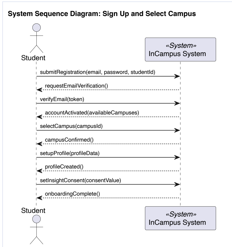
Figure 6.3: Original system sequence diagram - Sign Up and Select Campus.
