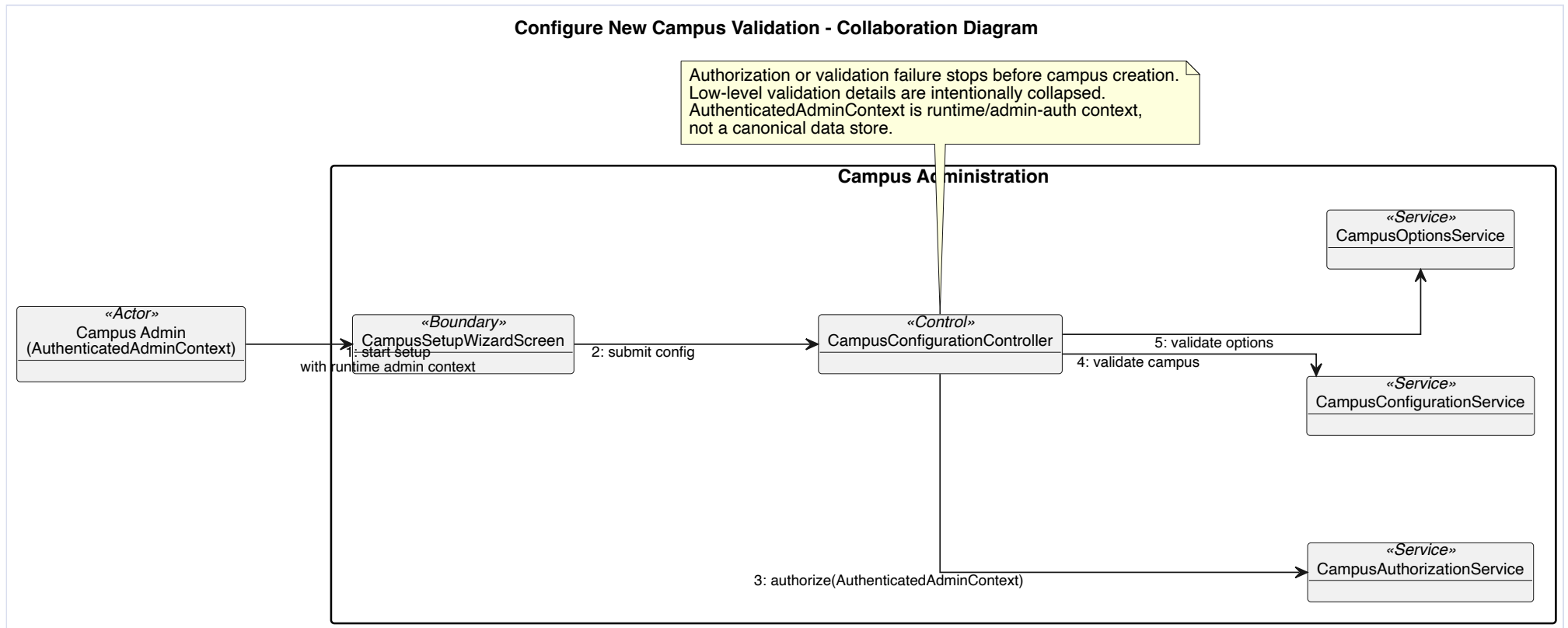
Figure 6.17: Original collaboration diagram - Configure New Campus.
