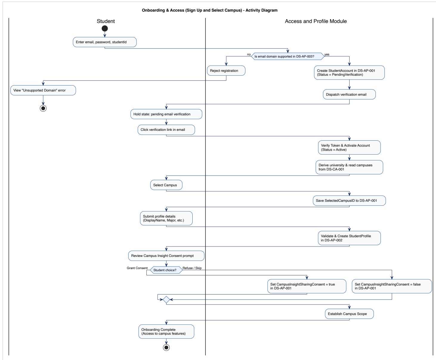
Appendix Figure H.7: Onboarding and Access Activity Diagram.
