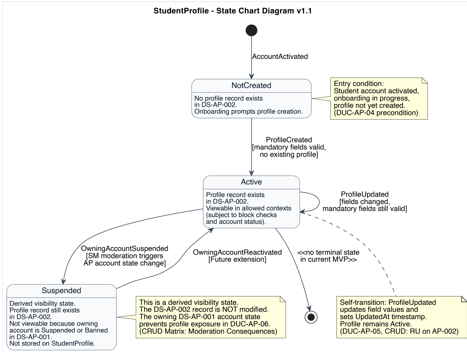
Figure 6.20: Original state chart - Student Profile.
