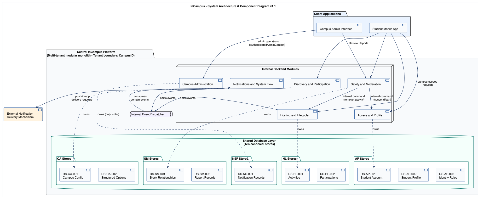
Appendix Figure H.6: Component Diagram.
