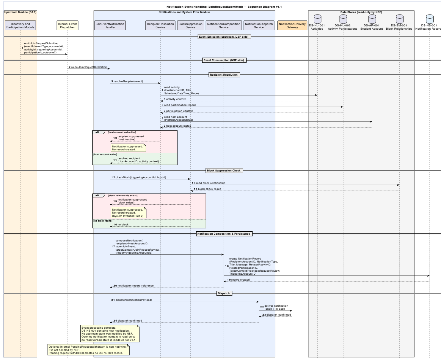
Appendix Figure H.13: Notification Event Handling Sequence Diagram.
