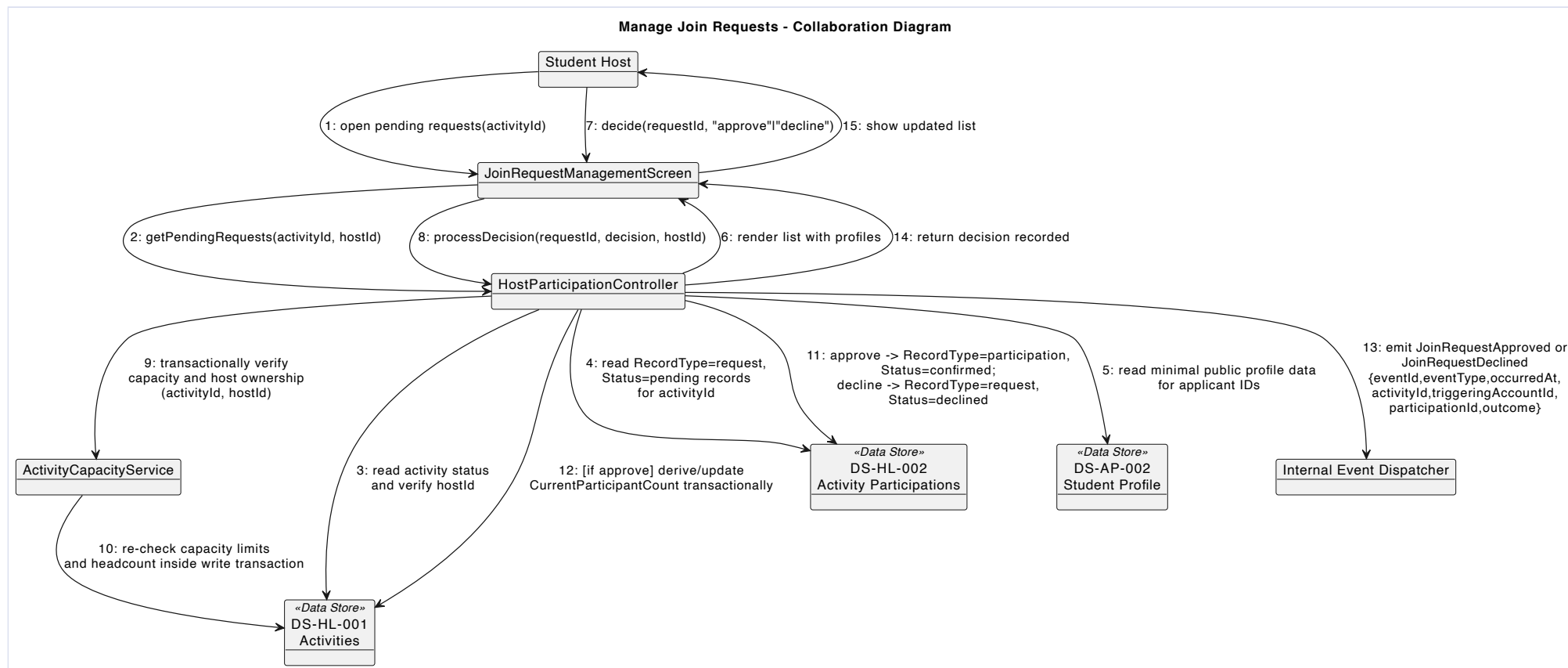
Appendix Figure H.18: Manage Join Requests Collaboration Diagram.
