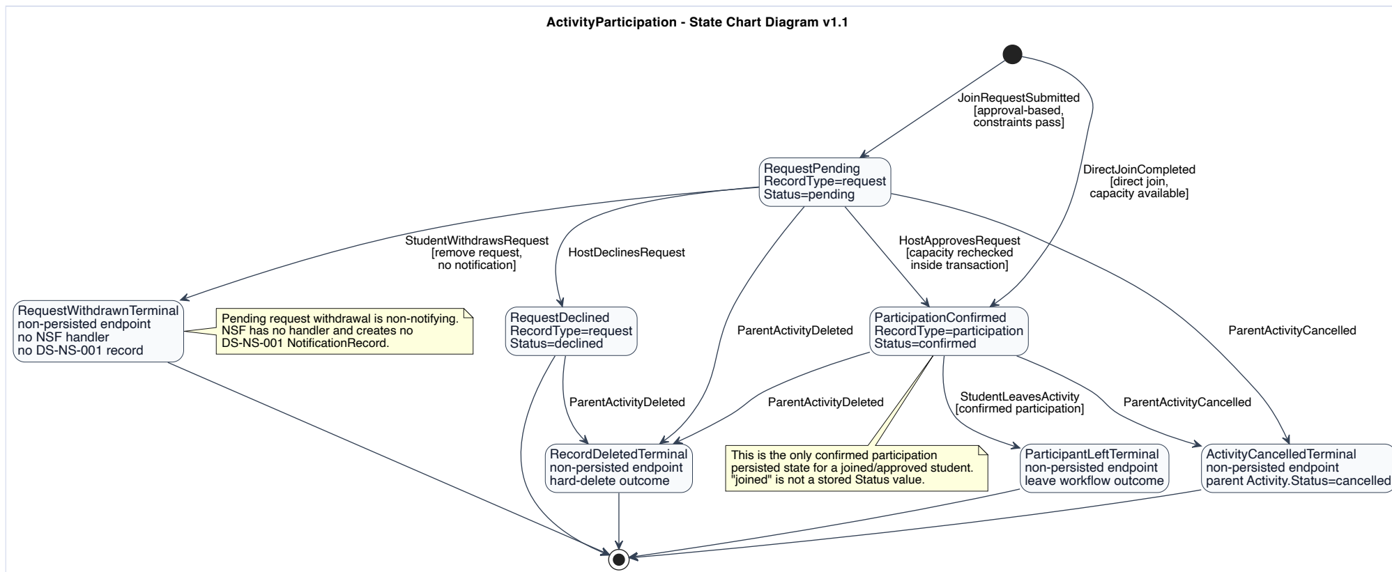
Appendix Figure H.24: Activity Participation State Chart.
