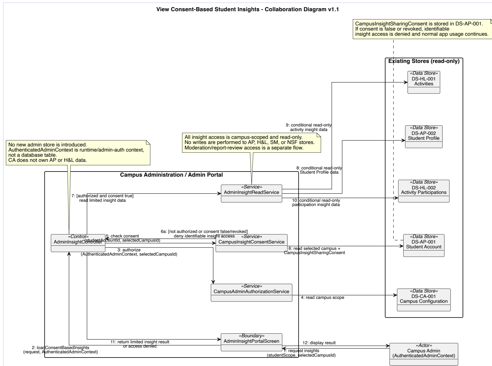
Appendix Figure H.23: Consent-Based Student Insights Collaboration Diagram.
