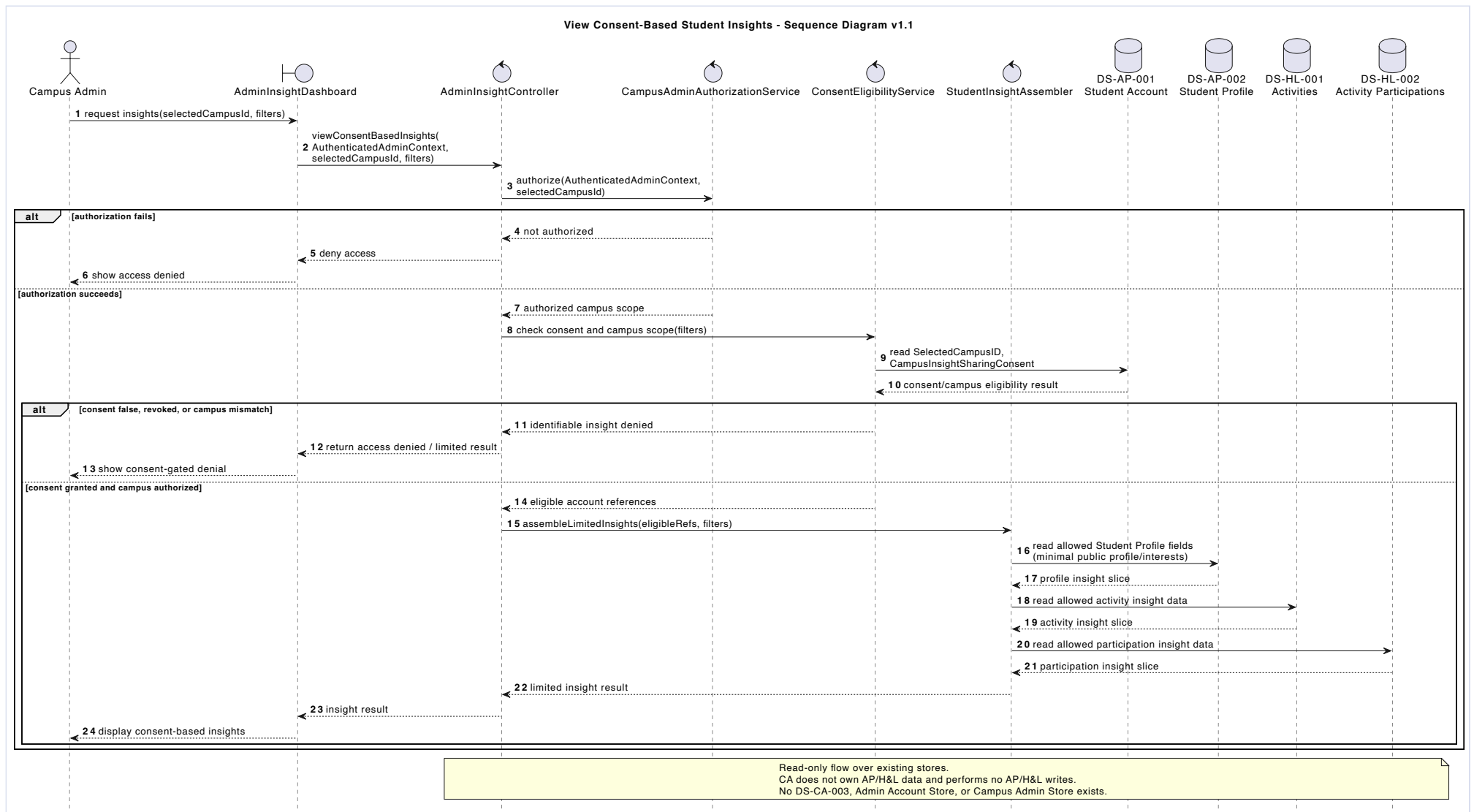
Appendix Figure H.16: View Consent-Based Student Insights Sequence Diagram.
