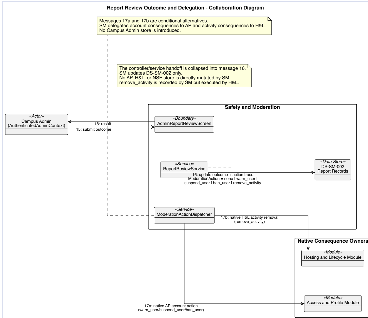
Figure 6.16: Original collaboration diagram - Report Review and Delegation.
