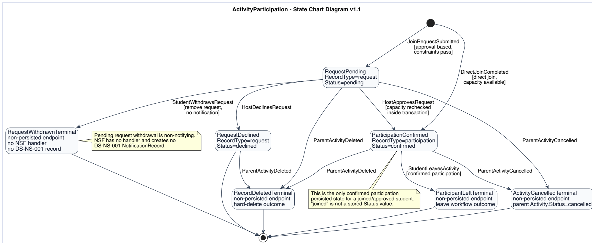
Figure 6.19: Original state chart - Activity Participation.
