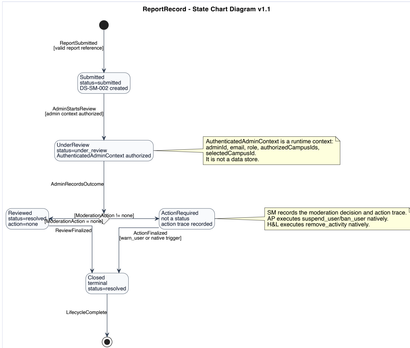
Appendix Figure H.26: Report Record State Chart.
