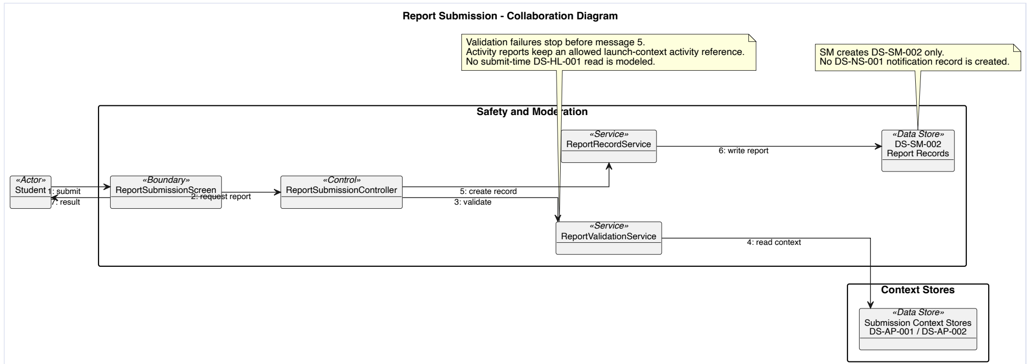
Figure 6.15: Original collaboration diagram - Report Submission.
