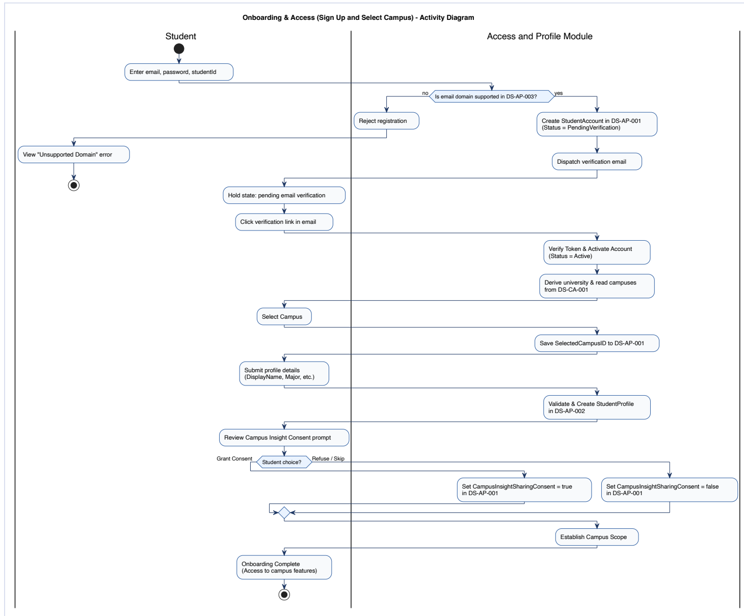
Figure 6.22: Original activity diagram - Onboarding and Access.
