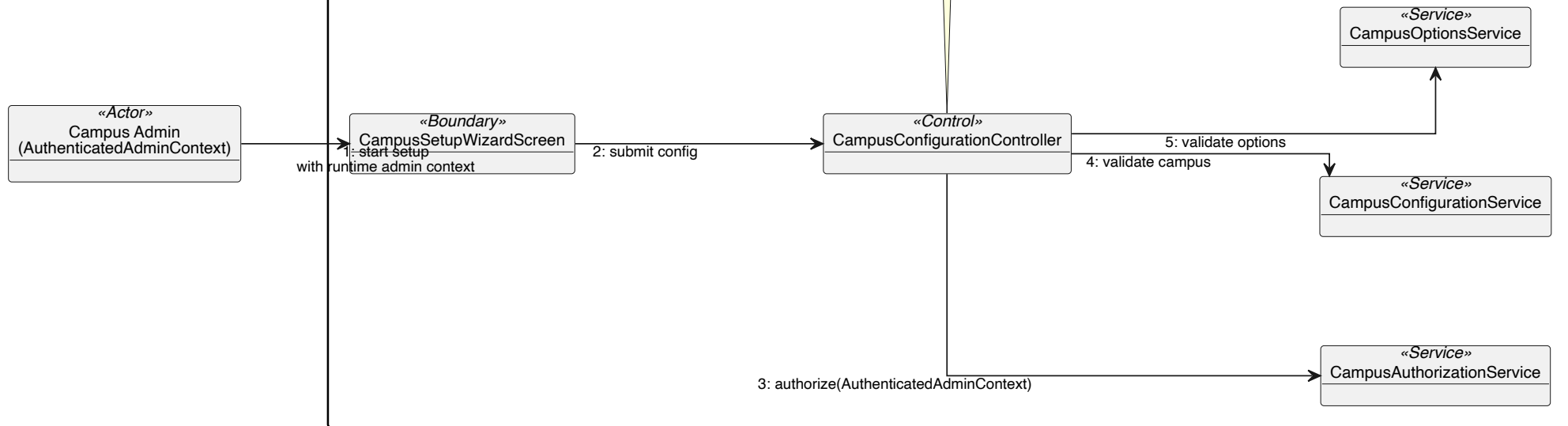
Appendix Figure H.22: Configure New Campus Collaboration Diagram.
