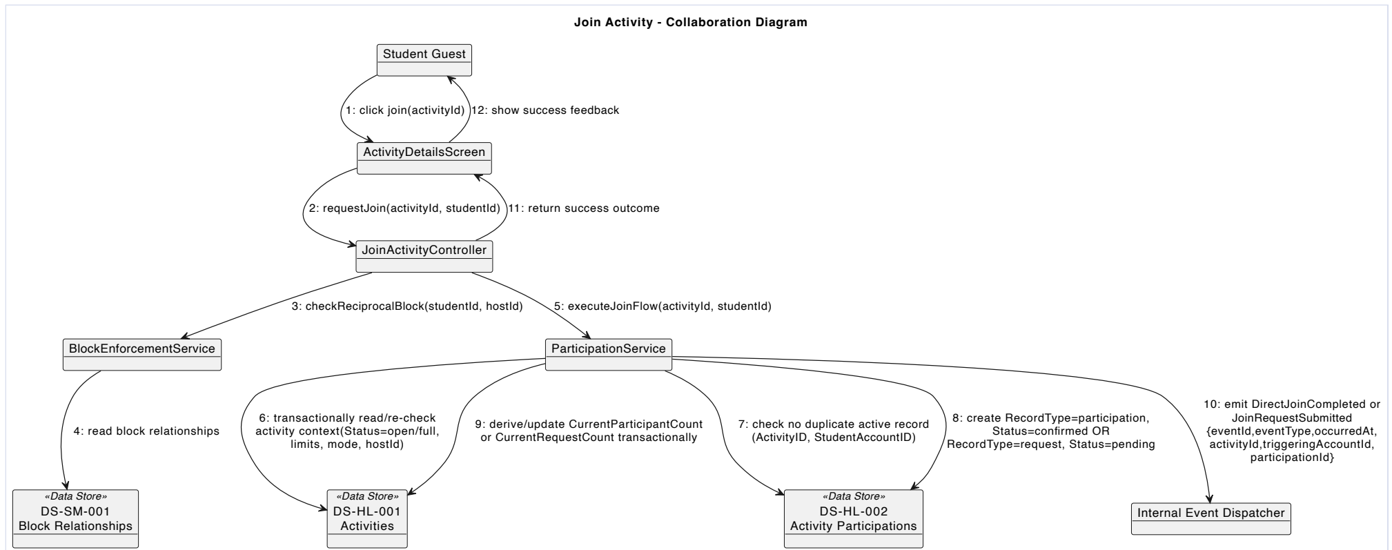
Appendix Figure H.17: Join Activity Collaboration Diagram.
