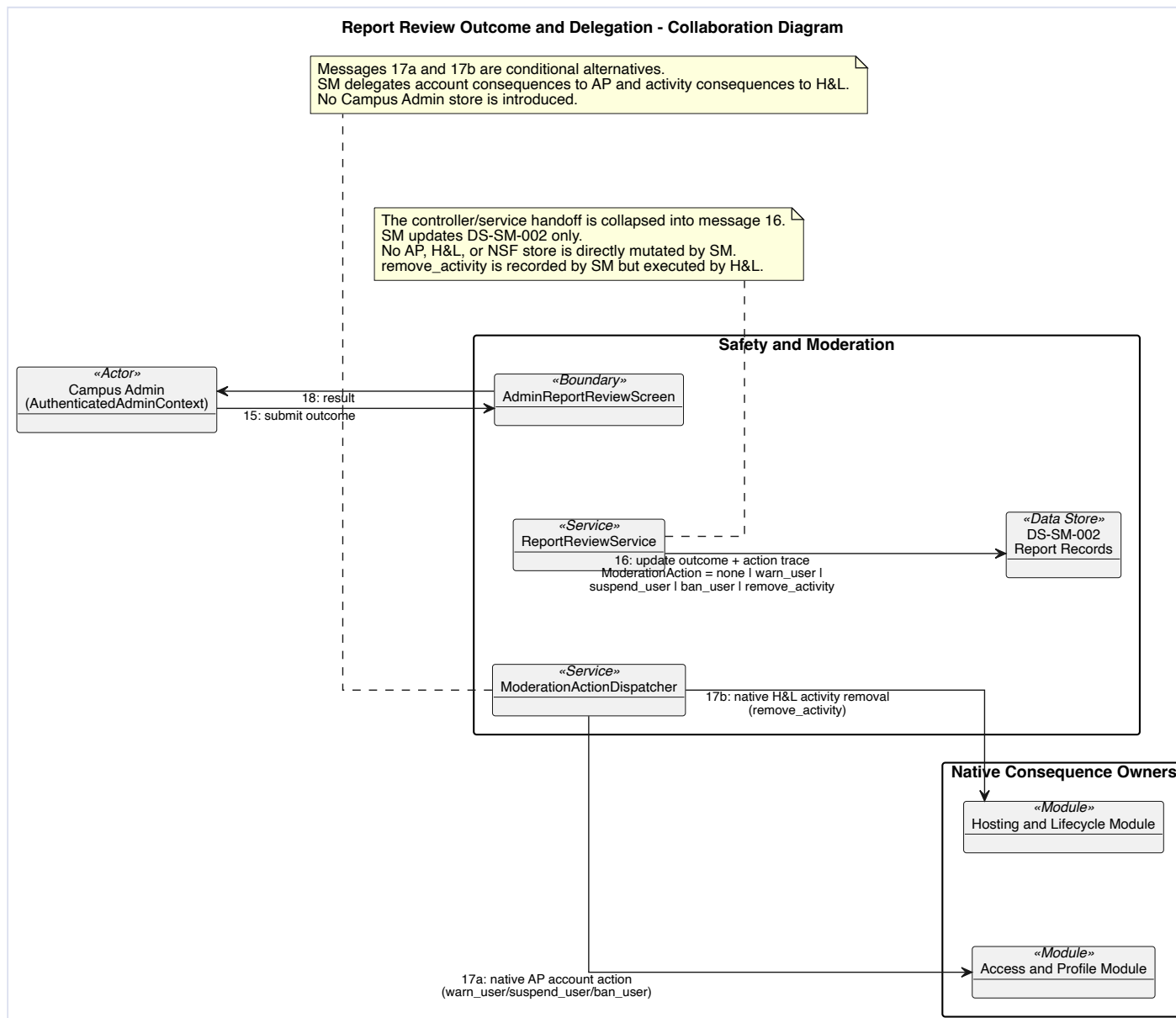
Appendix Figure H.21: Report Review and Delegation Collaboration Diagram.
