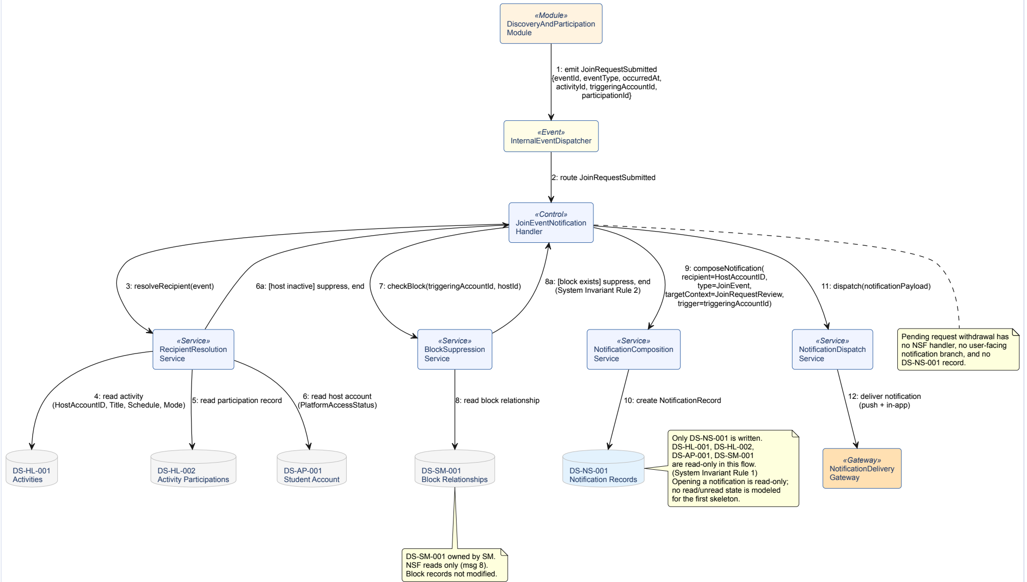
Appendix Figure H.19: Notification Event Handling Collaboration Diagram.
