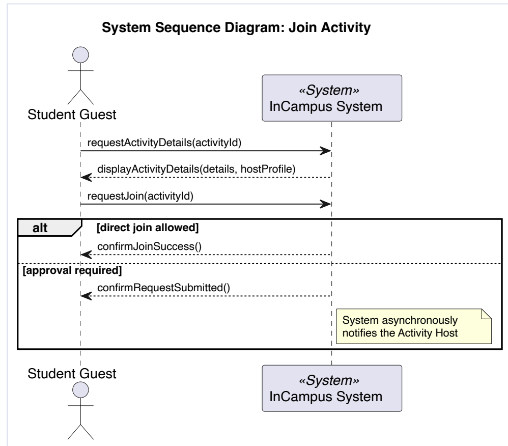
Figure 6.4: Original system sequence diagram - Join Activity.
