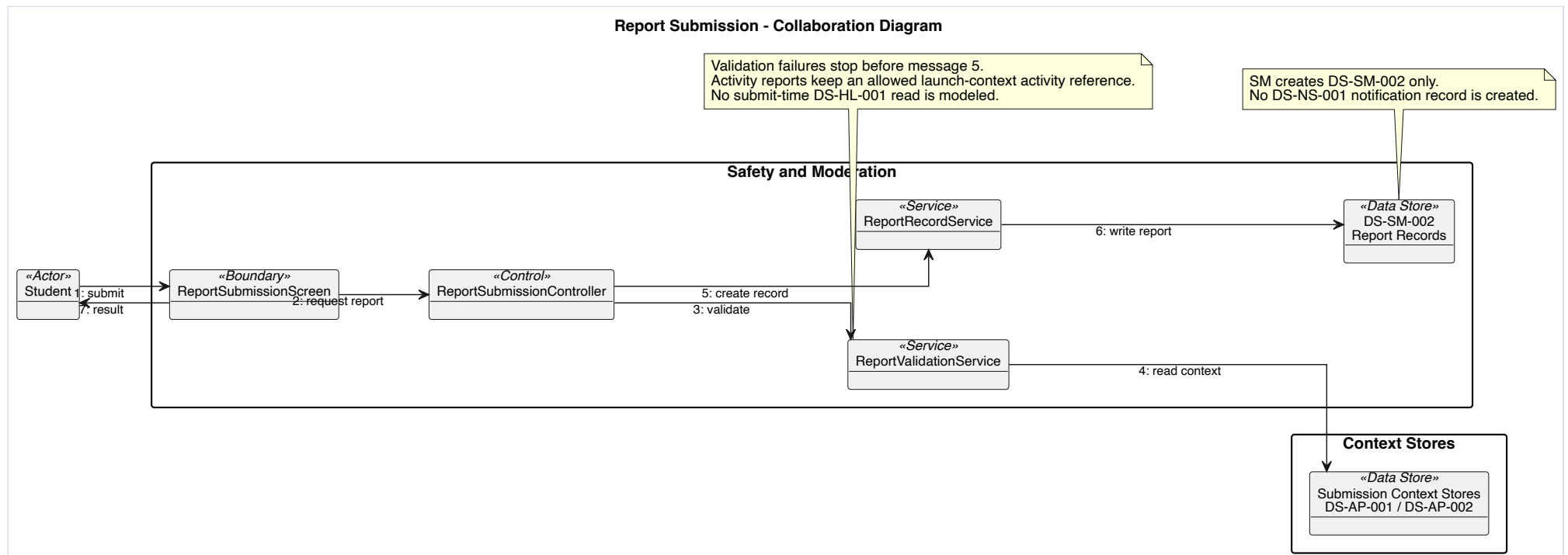
Appendix Figure H.20: Report Submission Collaboration Diagram.
