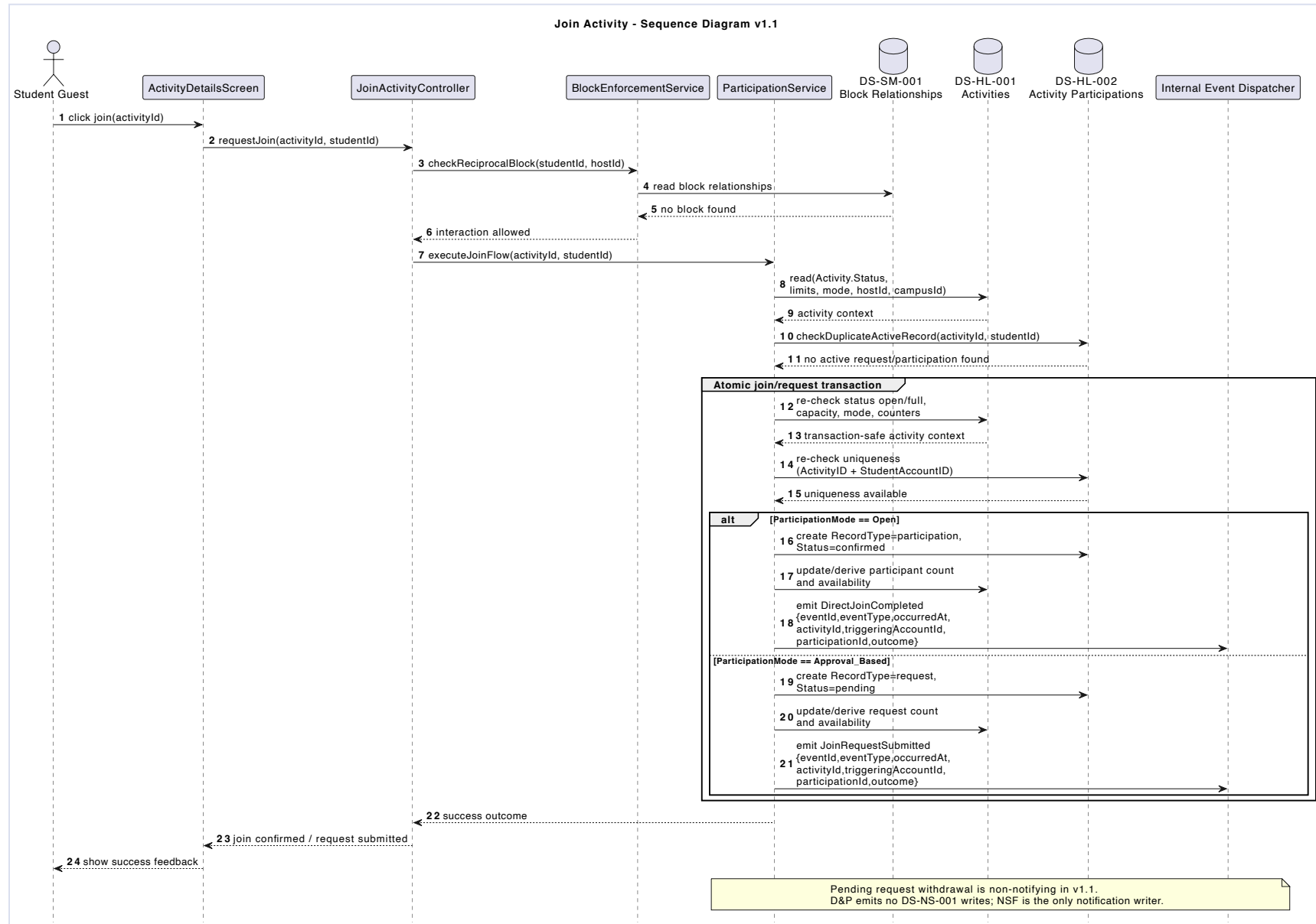
Figure 6.6: Original sequence diagram - Join Activity.
