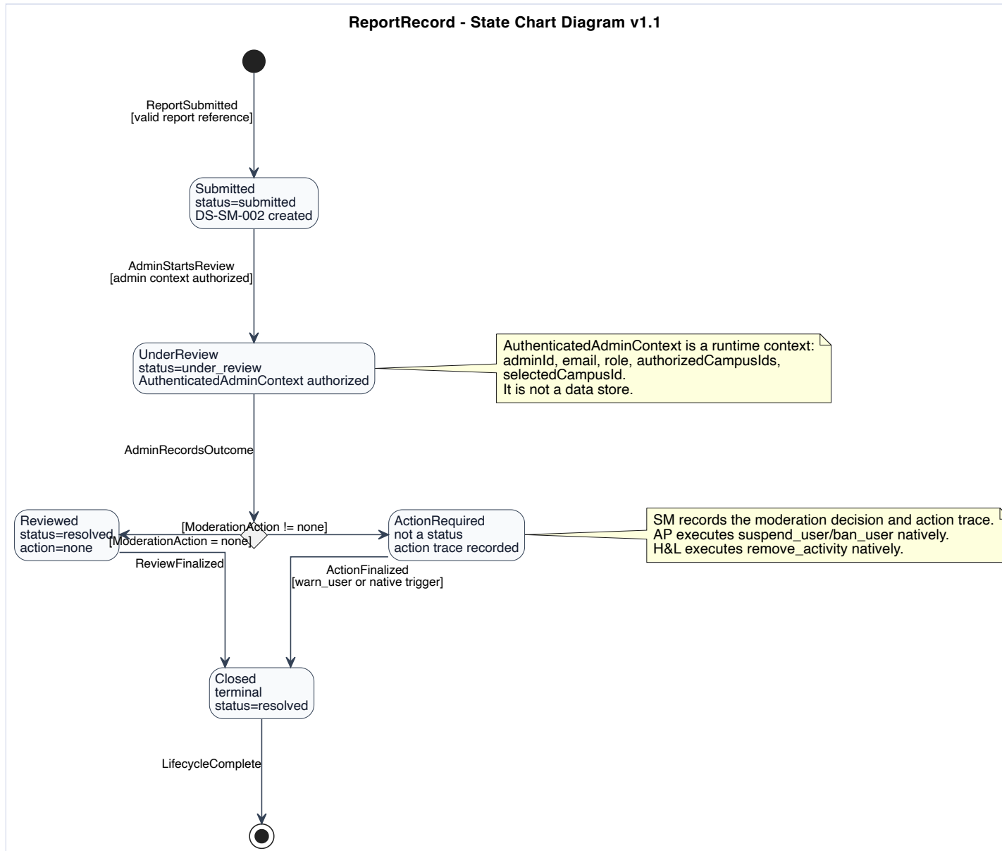
Figure 6.21: Original state chart - Report Record.
