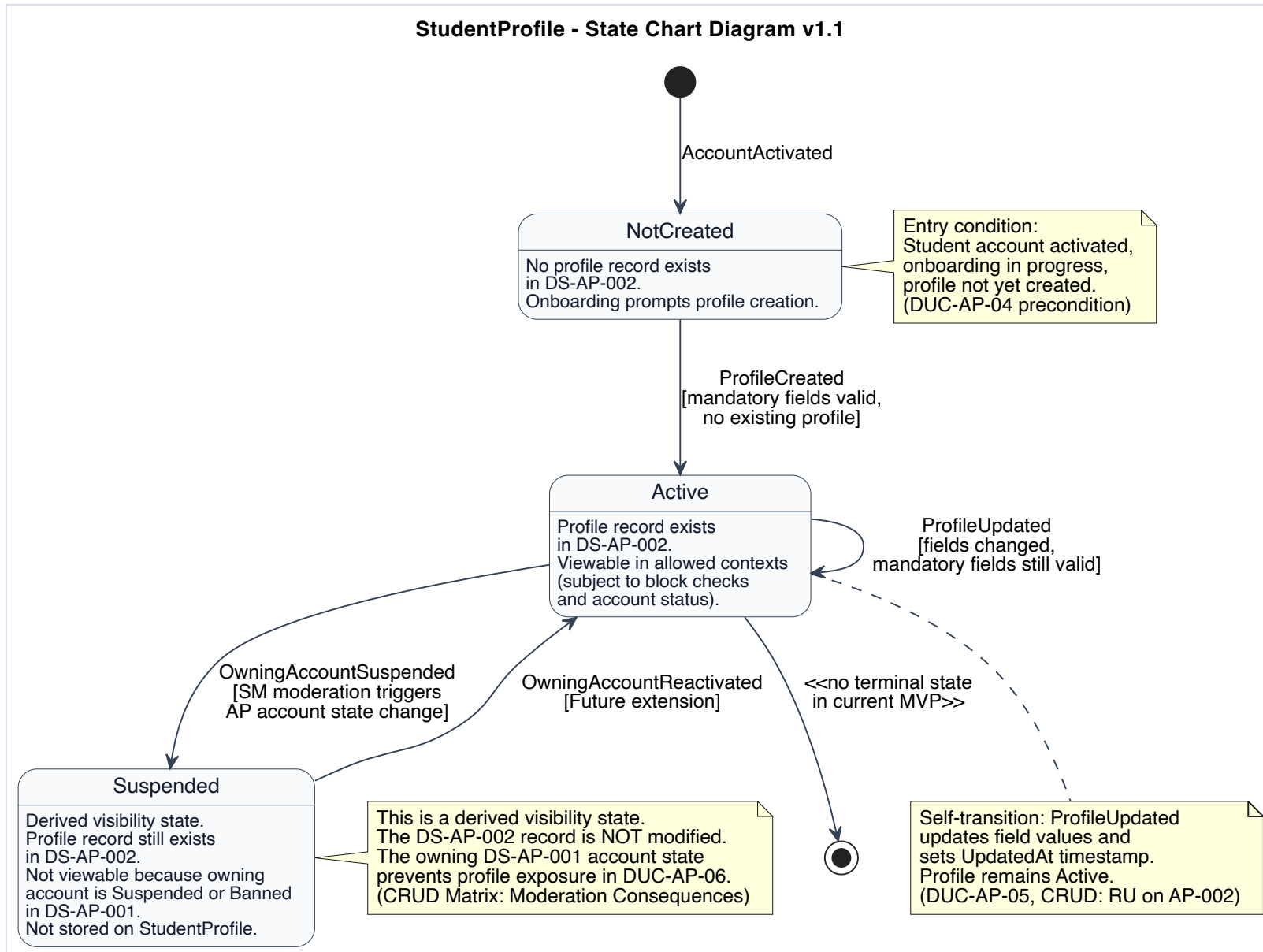
Appendix Figure H.25: Student Profile State Chart.
