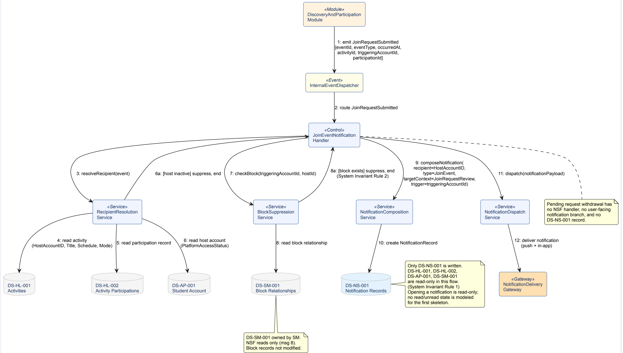
Figure 6.14: Original collaboration diagram - Notification Event Handling.
