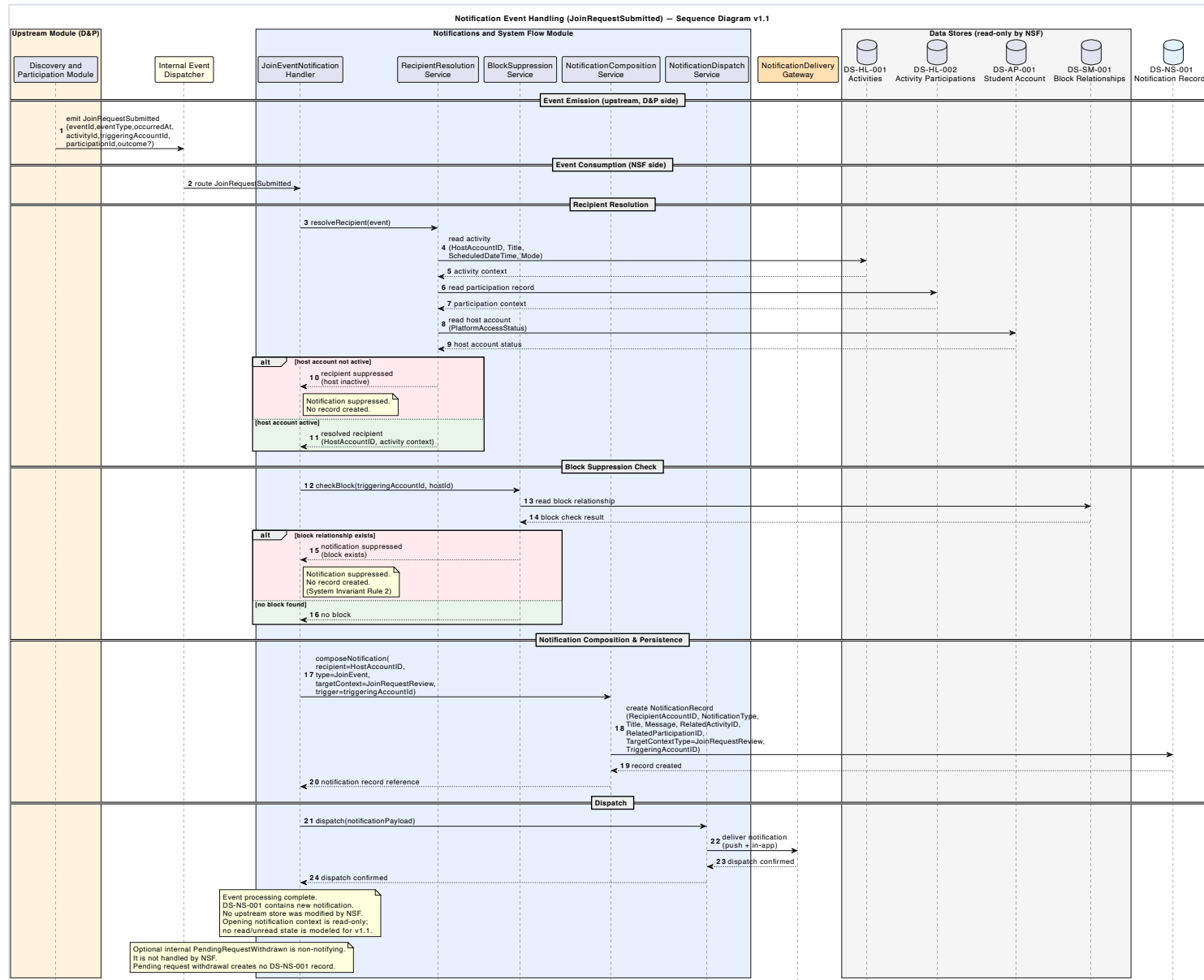
Figure 6.8: Original sequence diagram - Notification Event Handling.
