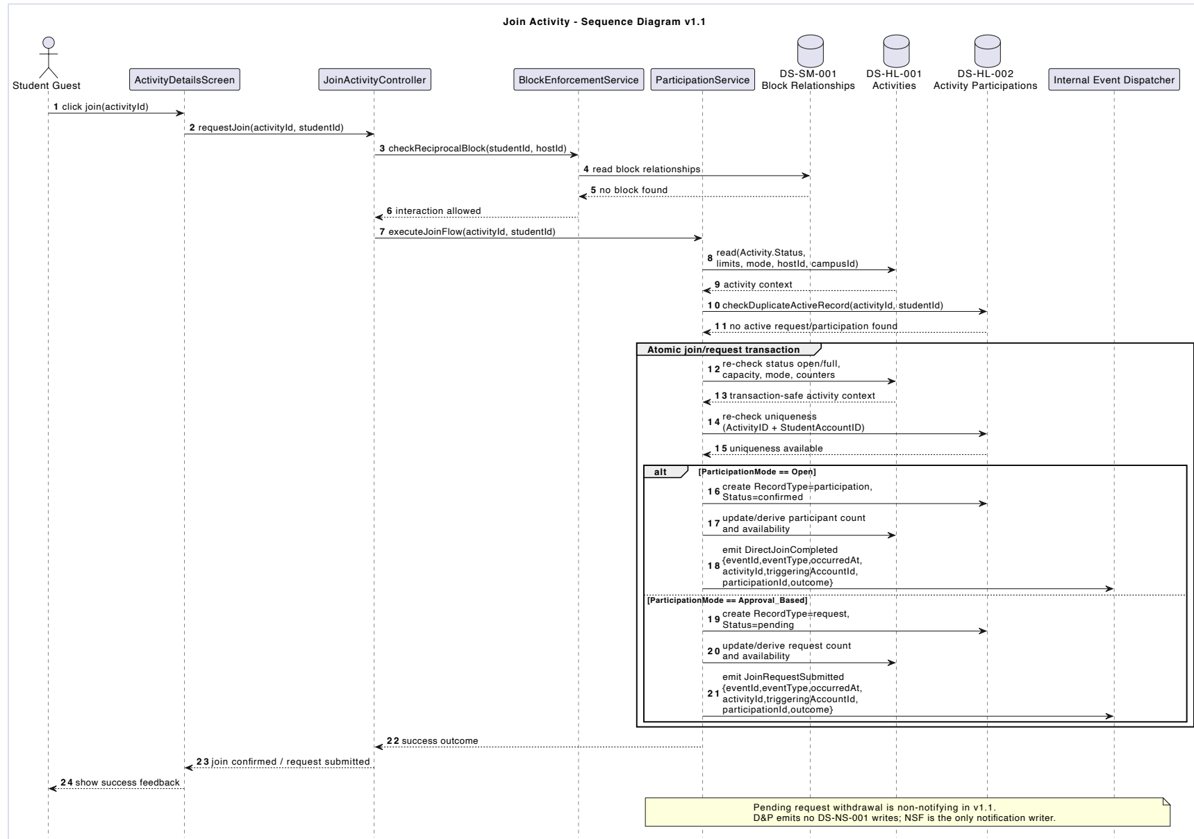
Appendix Figure H.11: Join Activity Sequence Diagram.
