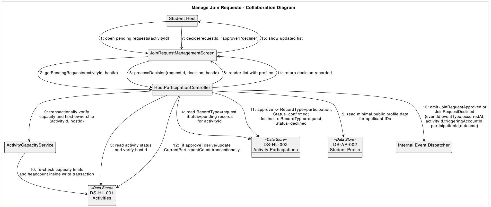
Figure 6.13: Original collaboration diagram - Manage Join Requests.
