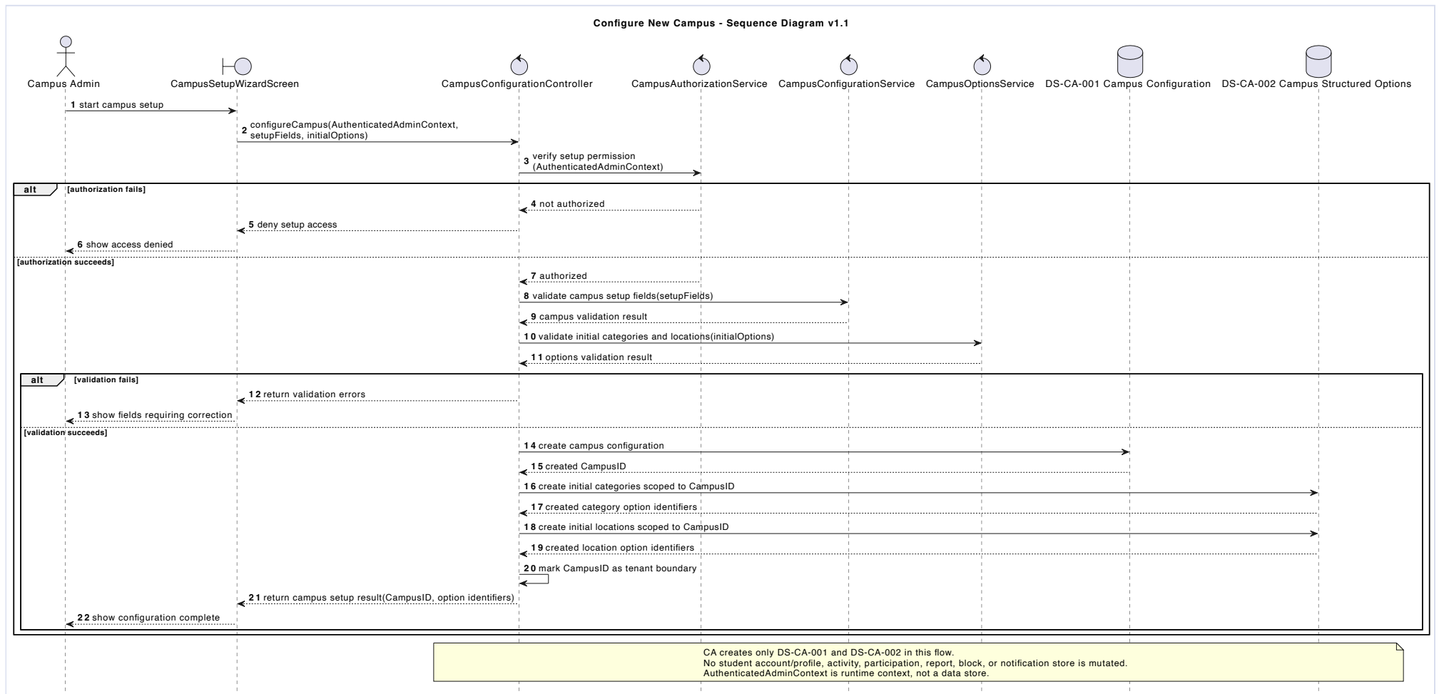
Figure 6.10: Original sequence diagram - Configure New Campus.
