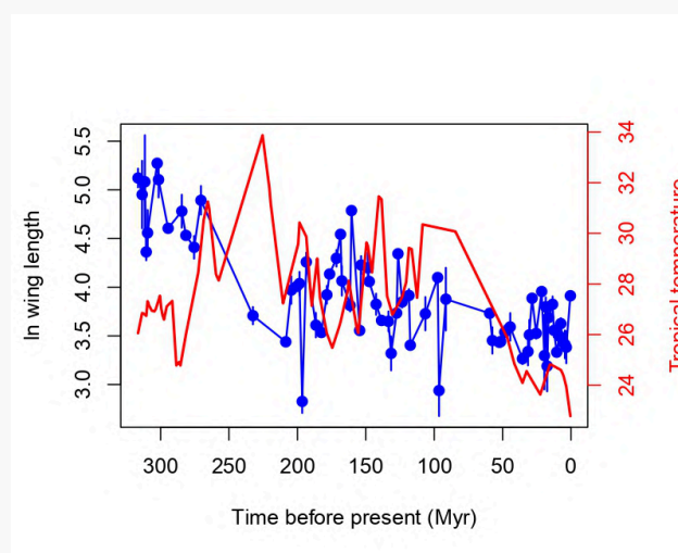
FIG 6 : Odonate wing size and tropical temperature through time. The blue line represents wing size (log in mm) and the red line represents temperature in degrees celsius. Both datasets are overlaid over each other so that we can visually see the negative correlation between them.
