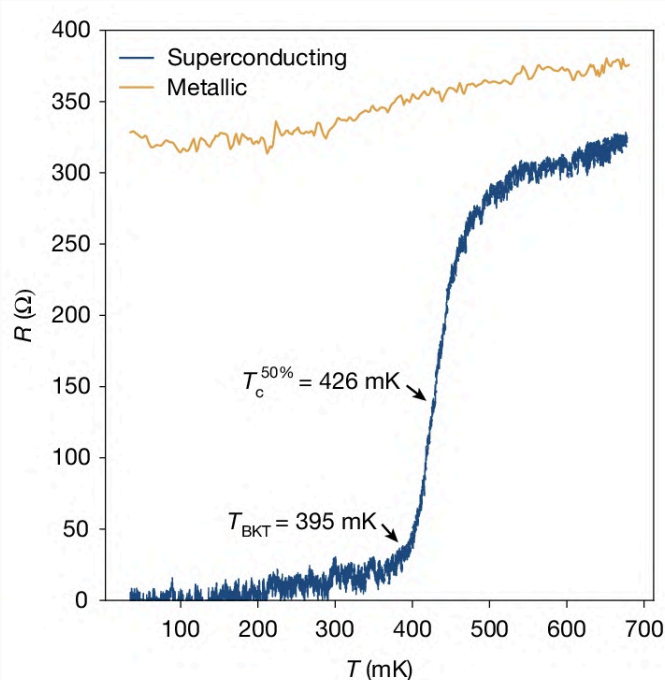
FIG (a) Resistance as a function of temperature, showing a clear drop to zero below the critical temperature at a specific twist angle, indicating the onset of a superconducting phase. FIG (b) Field-tuning at a fixed filling, illustrating a transition from an ordered magnetic phase into the superconducting dome.
