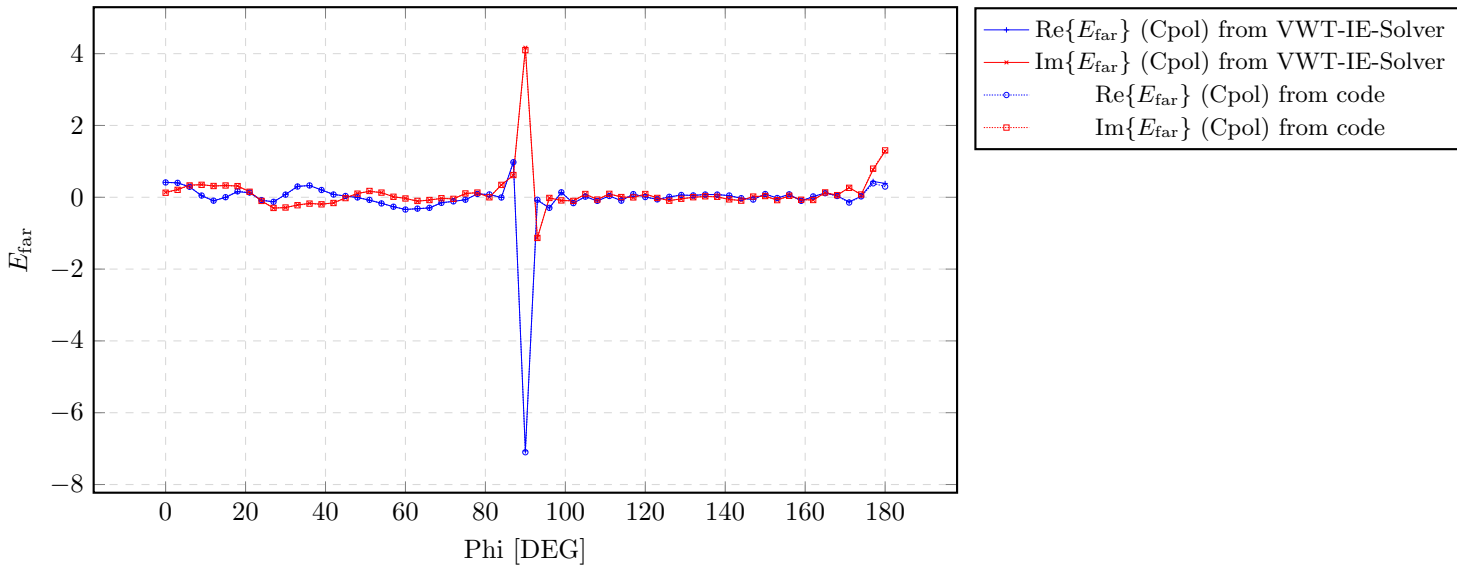
Monostatic Farfields
