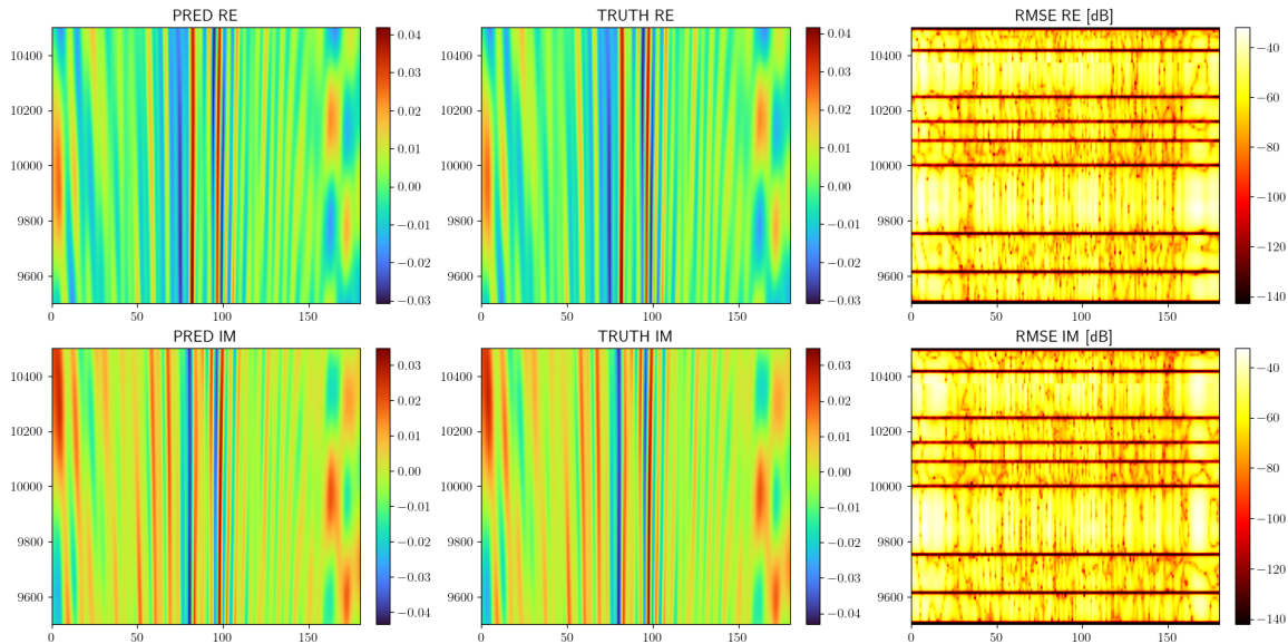
Figure: Prediction vs. Ground truth of monostatic farfields on PRIME aircraft
