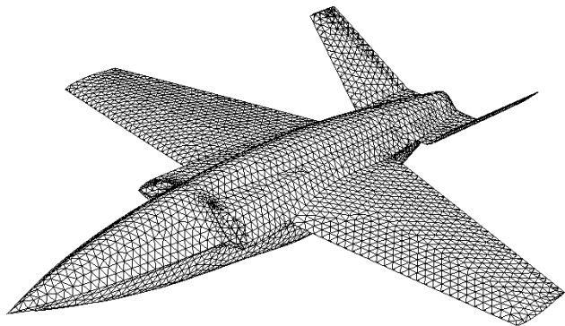
Figure: A schematic view of PRIME aircraft
