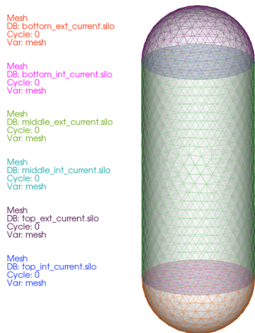
Figure: A schematic view of composite rounded cylinder
