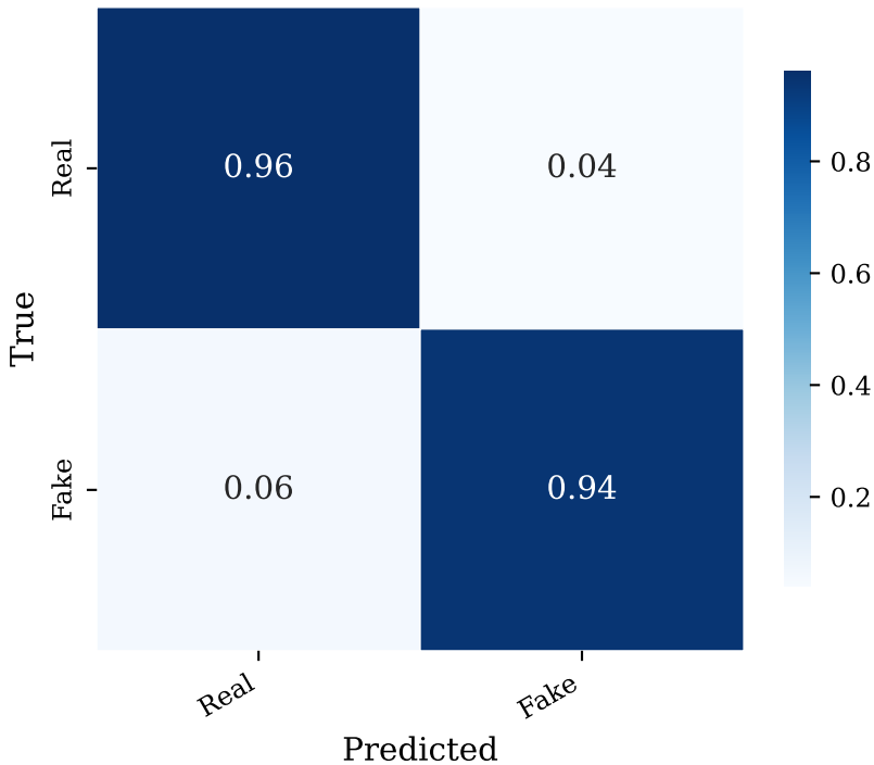
Confusion Matrix — FF++ Test
