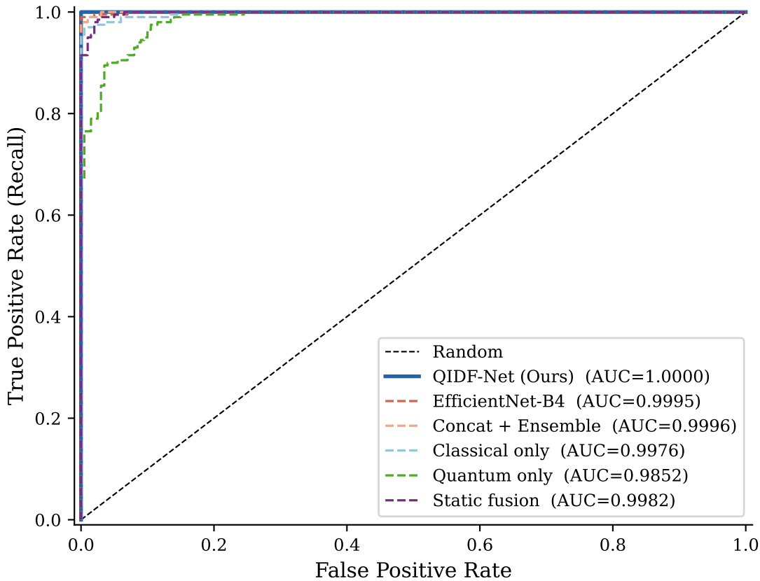
ROC Curves — FF++ Test Set
