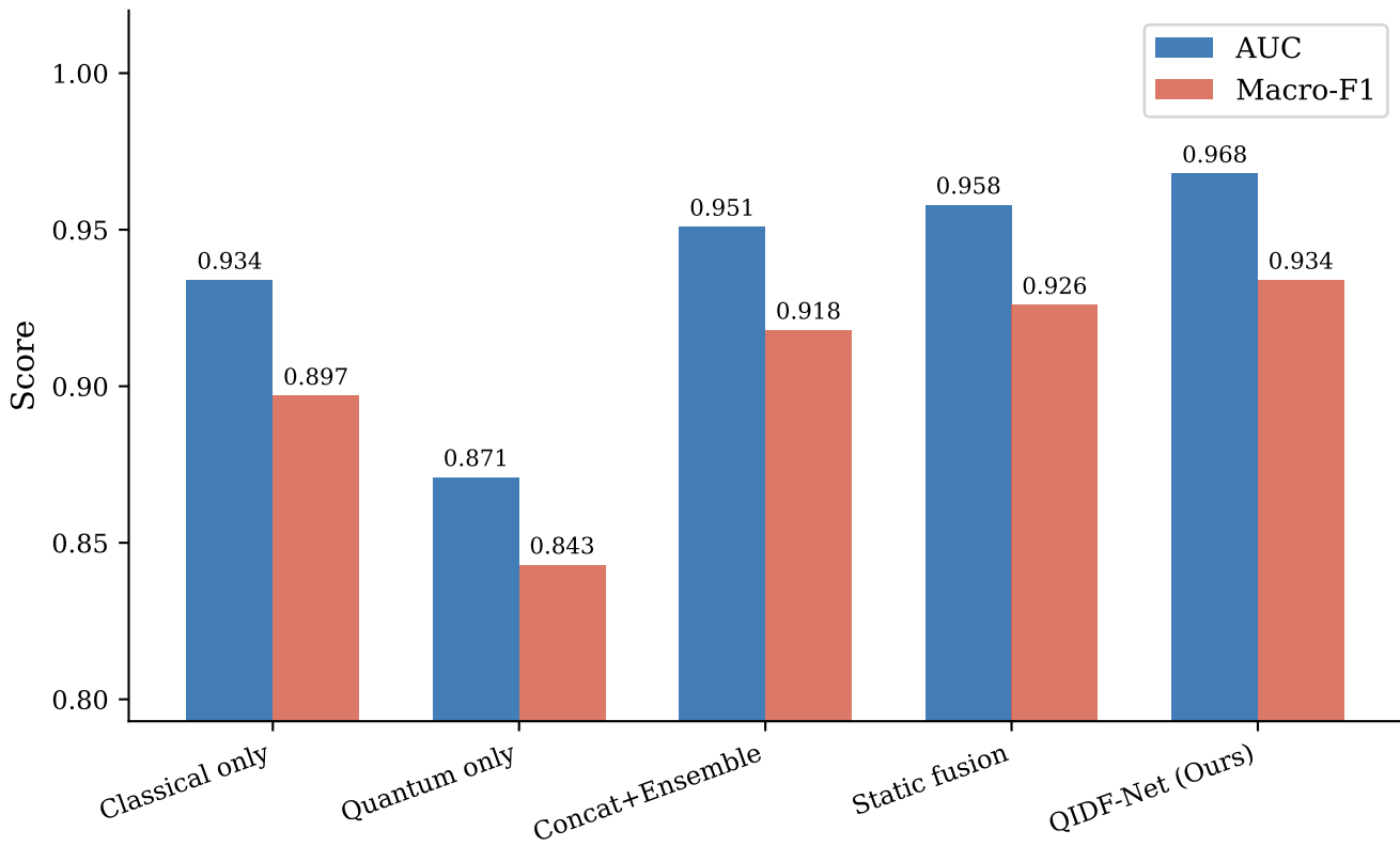
Ablation Study — Contribution of Each QIDF-Net Component
