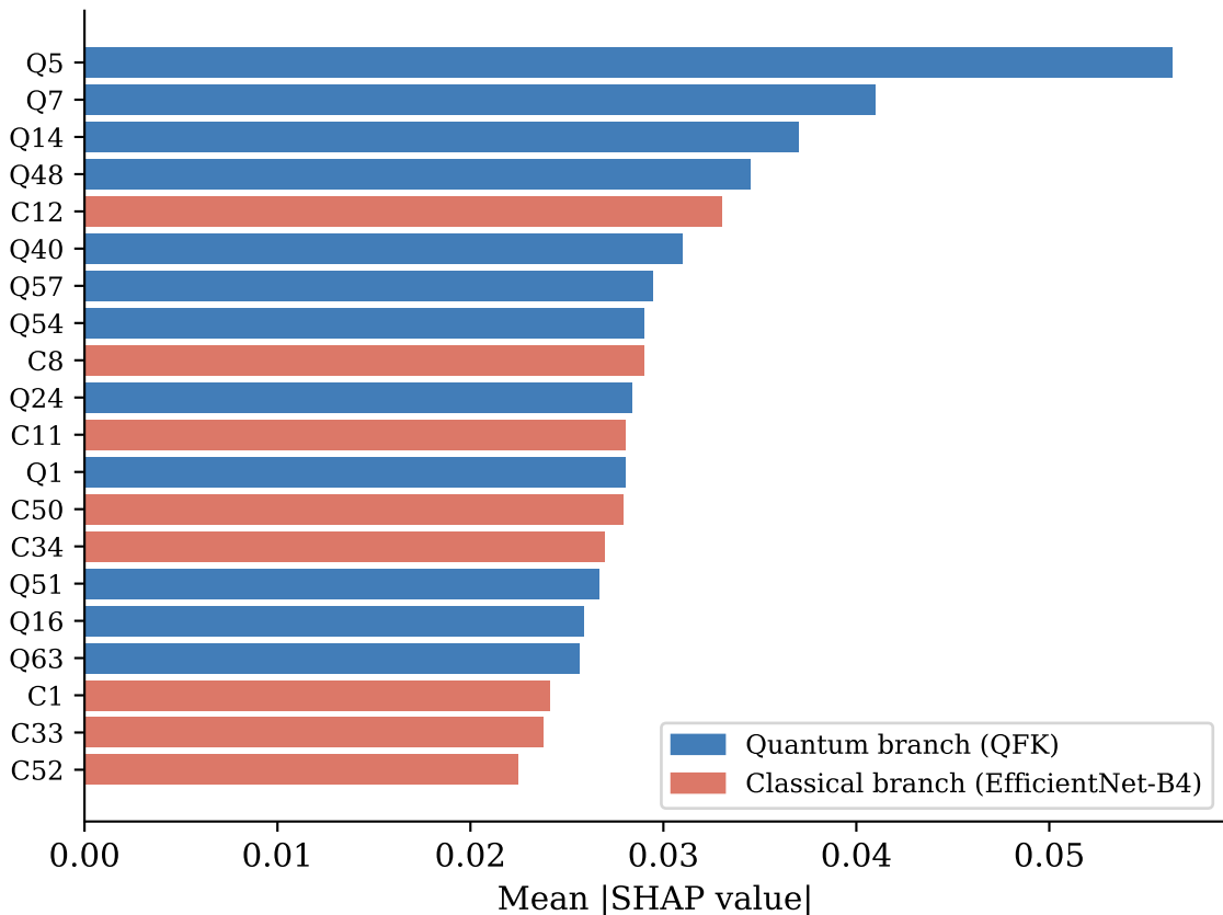
SHAP Feature Importance — Ensemble Detector (Q=Quantum branch, C=Classical branch)
